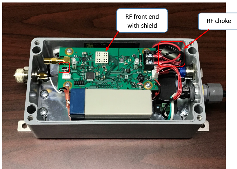
Figure 2 – Internal/Top View of Circuit Board
