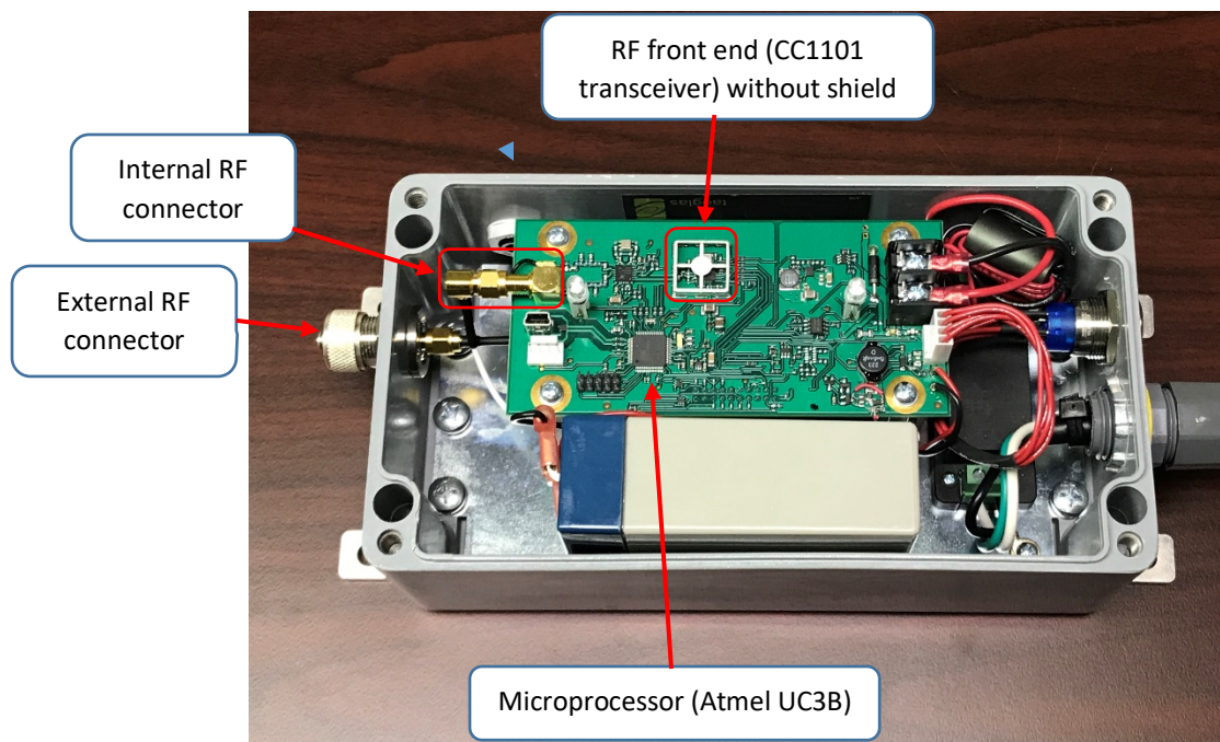
Figure 1 – Internal view of IMN
