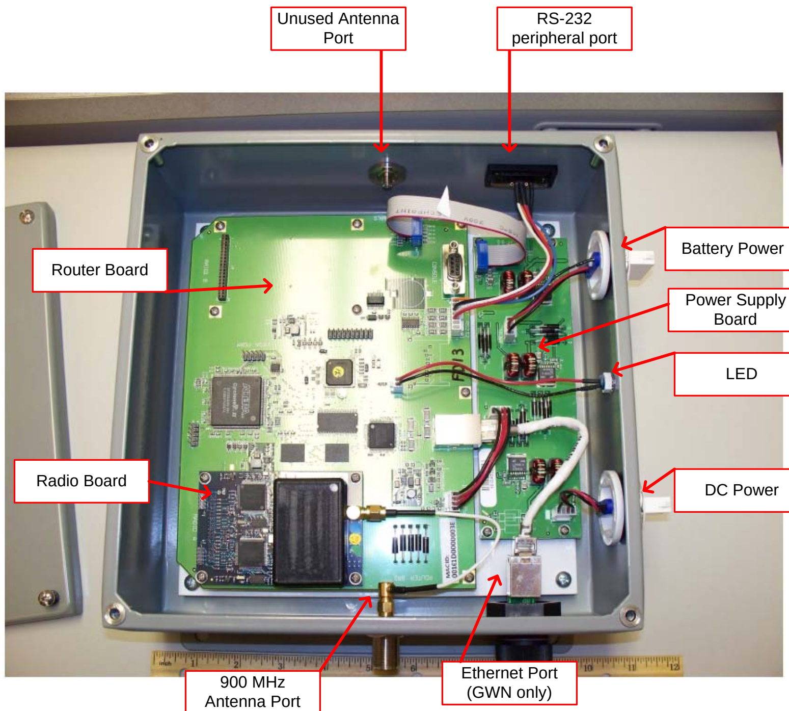
IWT GWN/FMN INTERNAL VIEW
