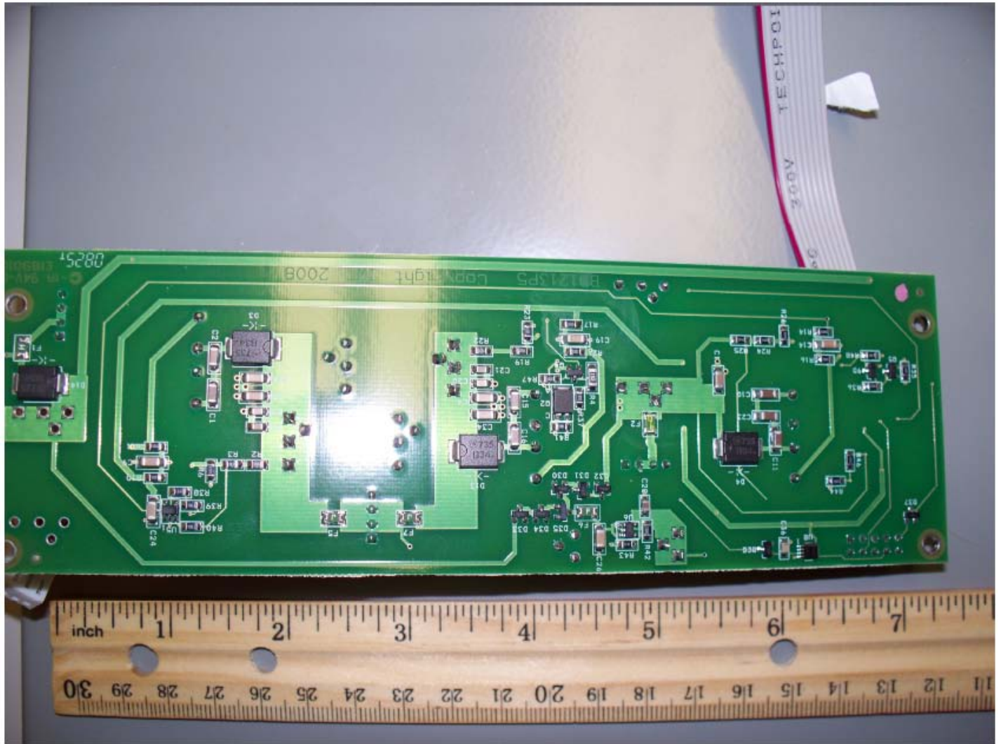
IWT GWN/FMN POWER SUPPLY BOARD BOTTOM VIEW
