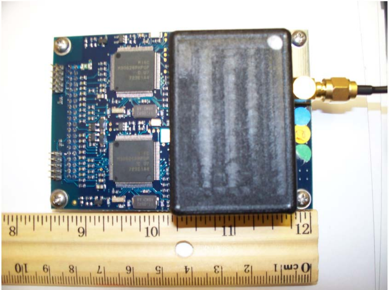
IWT GWN/FMN 900 MHz RADIO BOARD TOP VIEW
