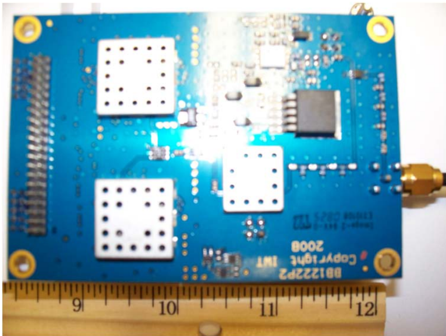
IWT GWN/FMN 900 MHz RADIO BOARD BOTTOM VIEW
