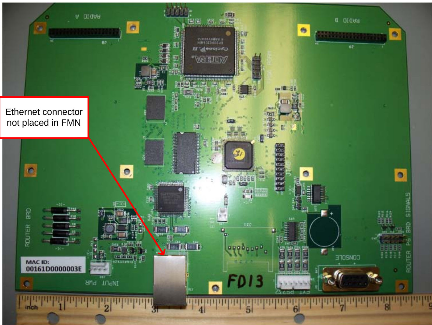
IWT GWN/FMN ROUTER BOARD TOP VIEW
