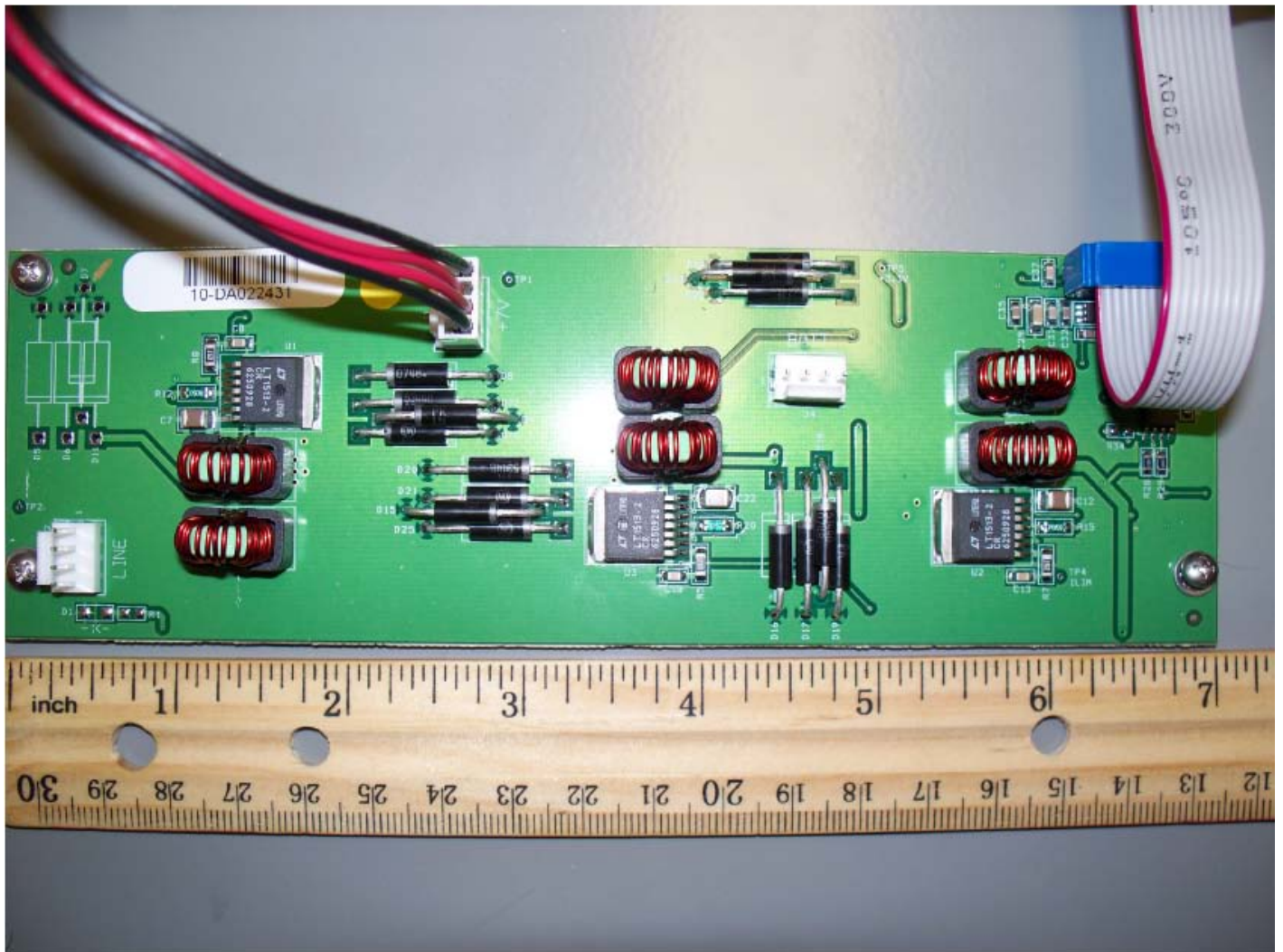
IWT GWN/FMN POWER SUPPLY BOARD TOP VIEW
