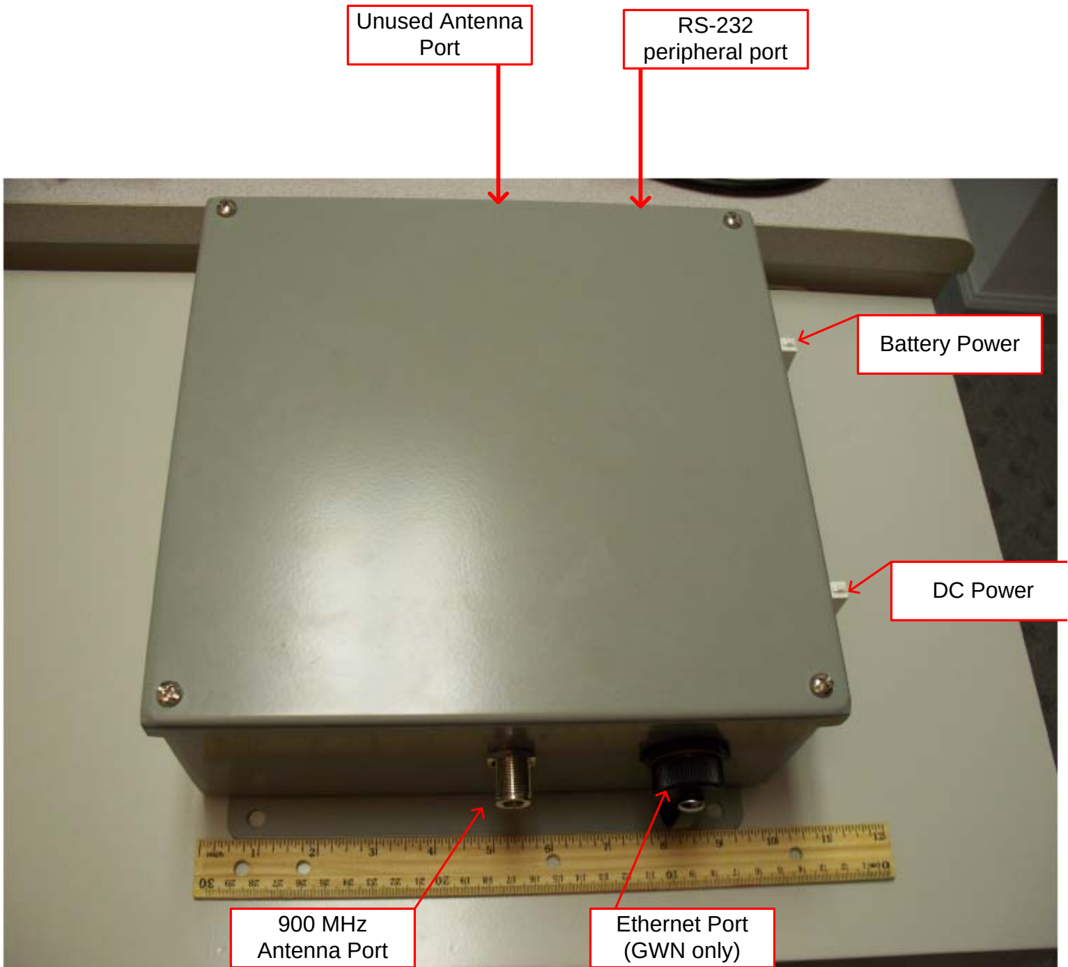
IWT GWN/FMN EXTERNAL WITH COVER
