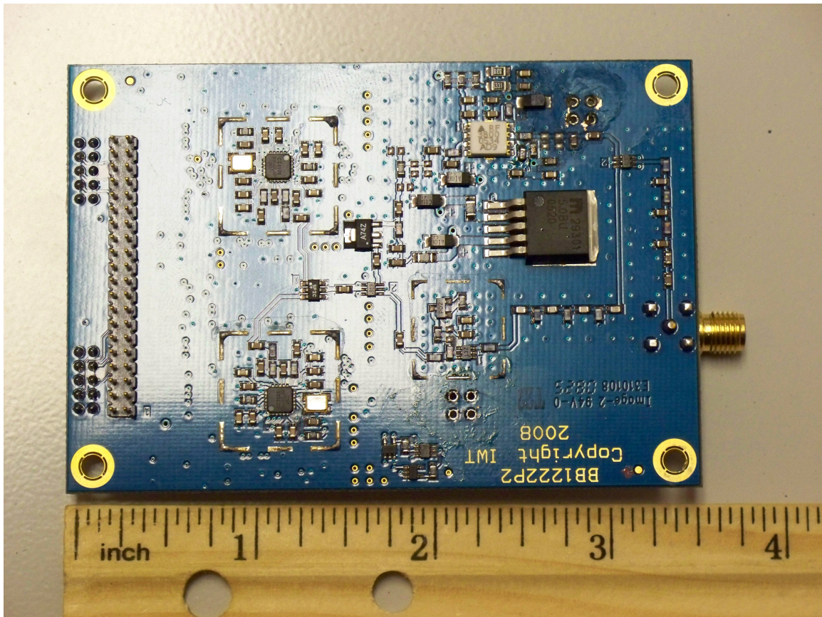
IWT GWN/FMN 900 MHz RADIO BOARD BOTTOM VIEW
