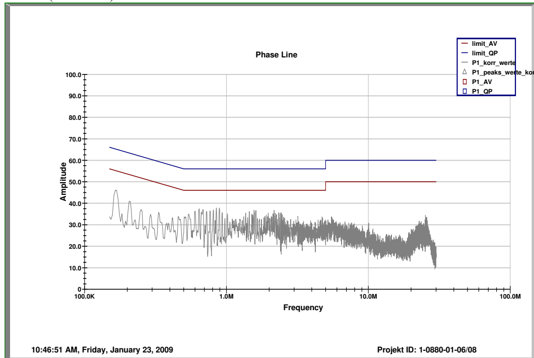
Plot 3: Phase Line (Idle-Mode)
