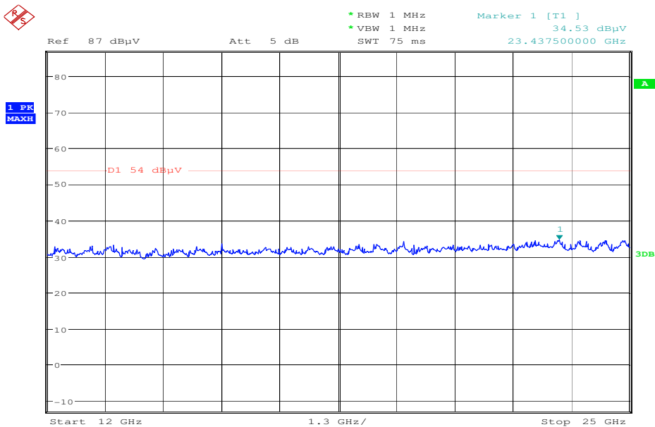
Plot 3: 12 - 25 GHz (valid for all channels)
