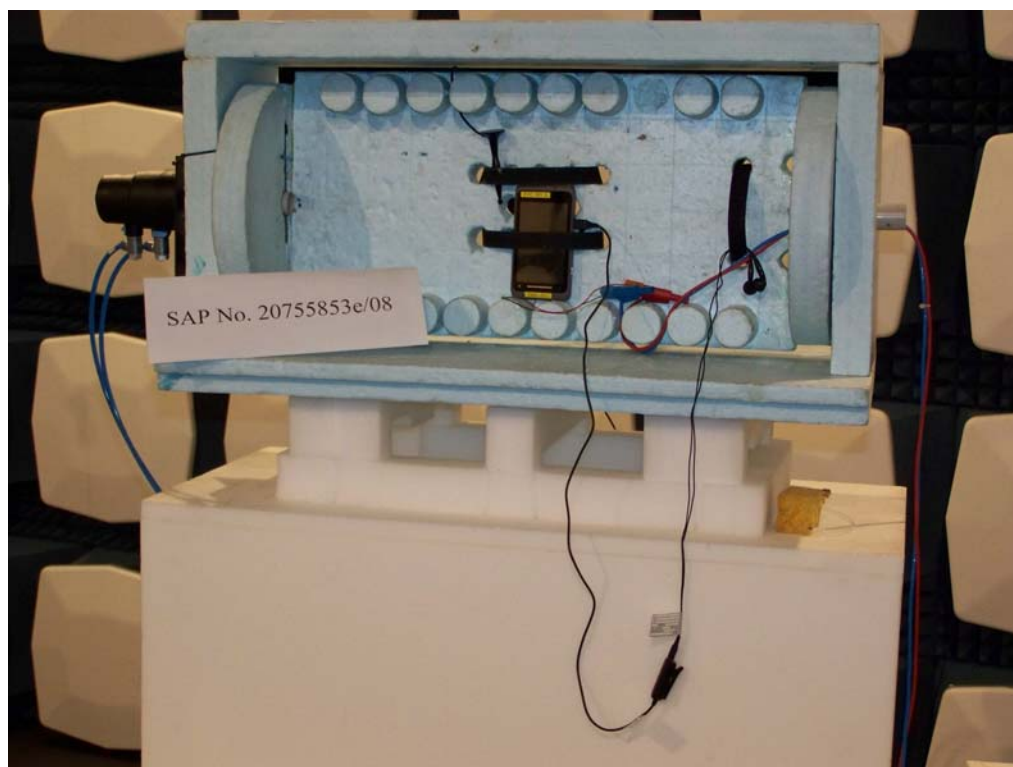
Photograph 2: radiated set-up
