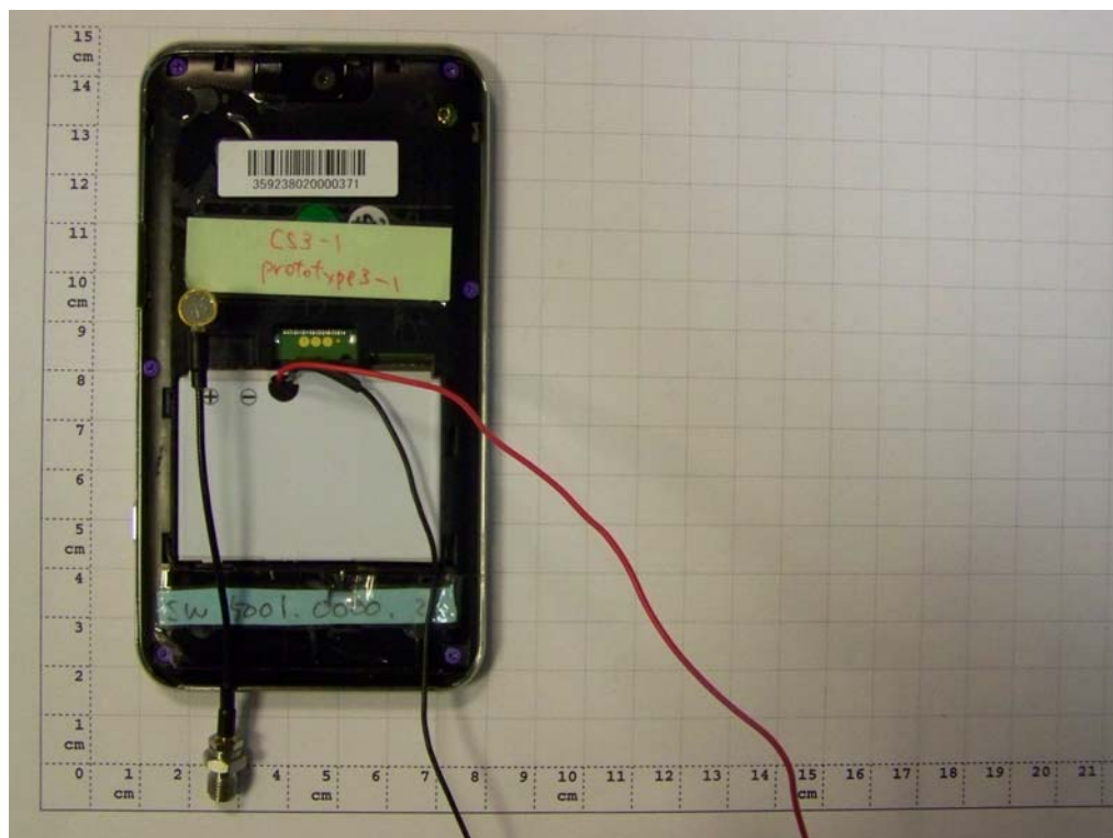
Photograph 1: conducted set-up: RF-adaptor and dummy battery
