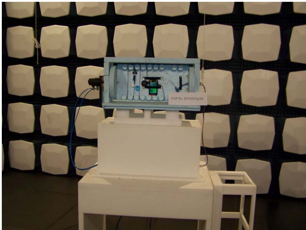
Photograph 2: radiated set-up
