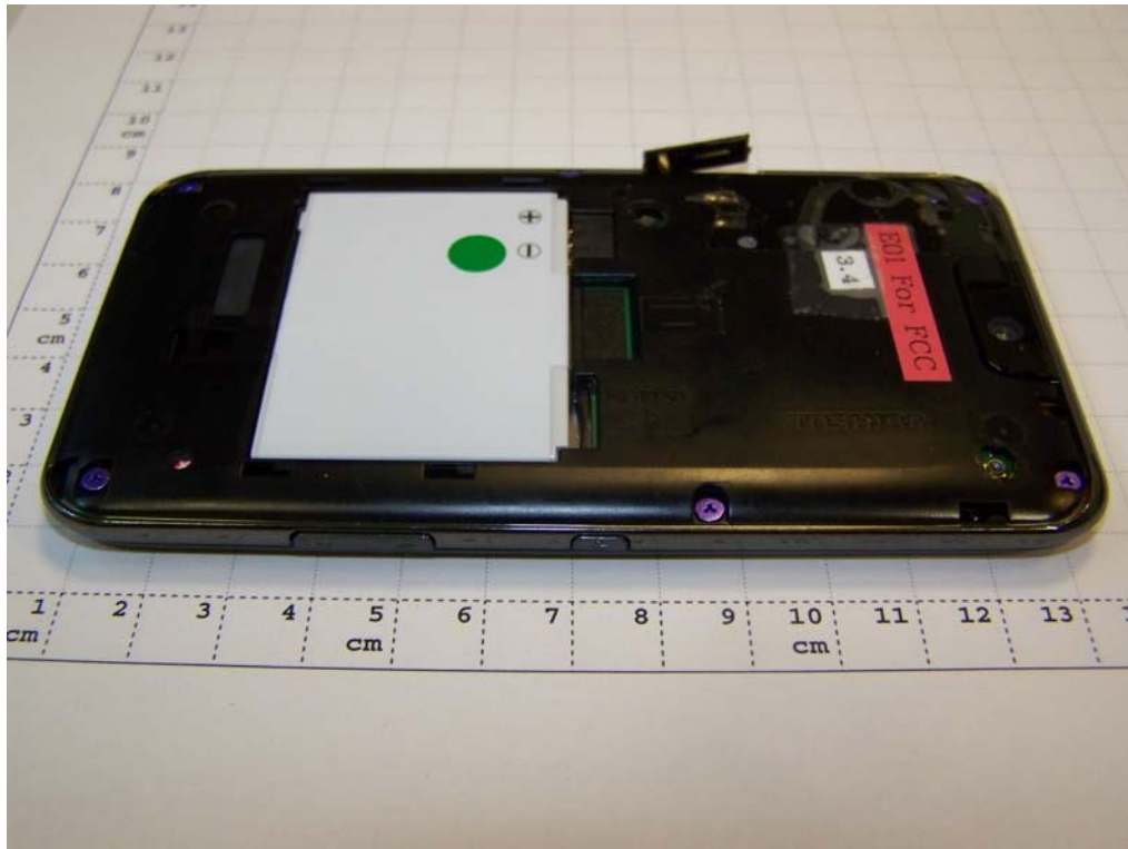
Photograph 5: Equipment under test: EUT A – right side
