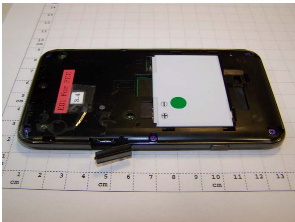
Photograph 4: Equipment under test: EUT A – right side
