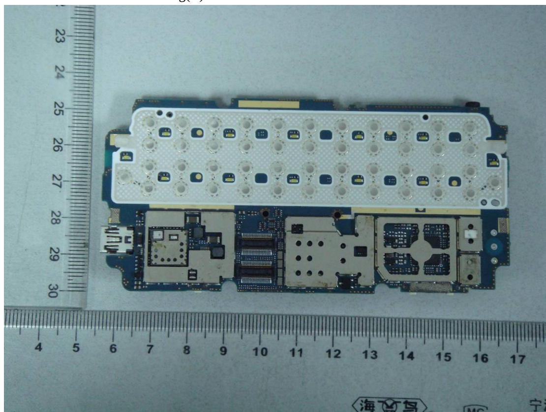
4. Main PCB without shielding(B)
