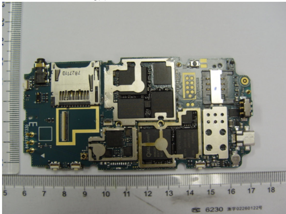
3. Main PCB without shielding(A)
