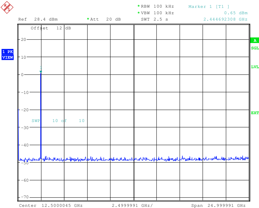
Plot 2: (DSSS)
