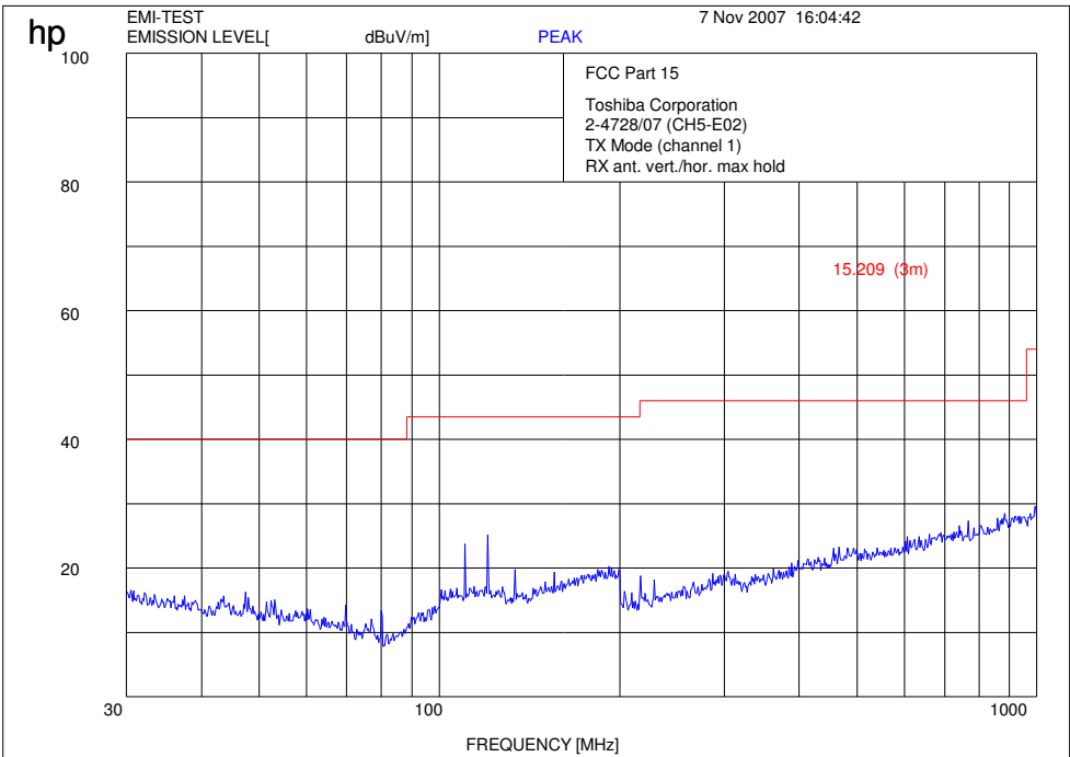
Plot 11: 0.03 - 1 GHz (lowest channel) (g Mode – 54 Mbps)
