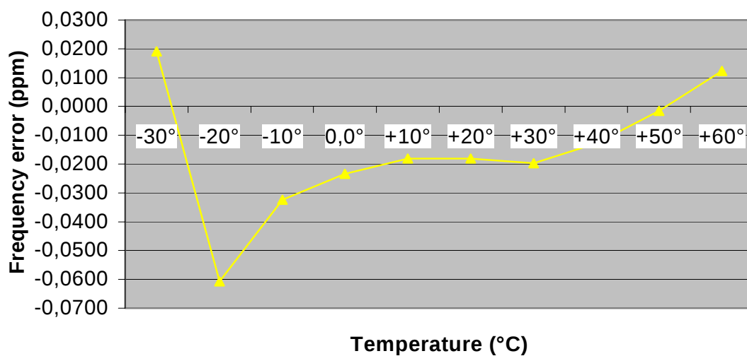
FREQUENCY ERROR VERSUS TEMPERATURE
