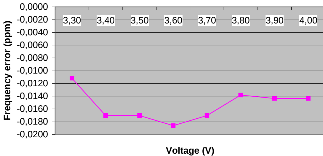
Frequency Error vs. Voltage
