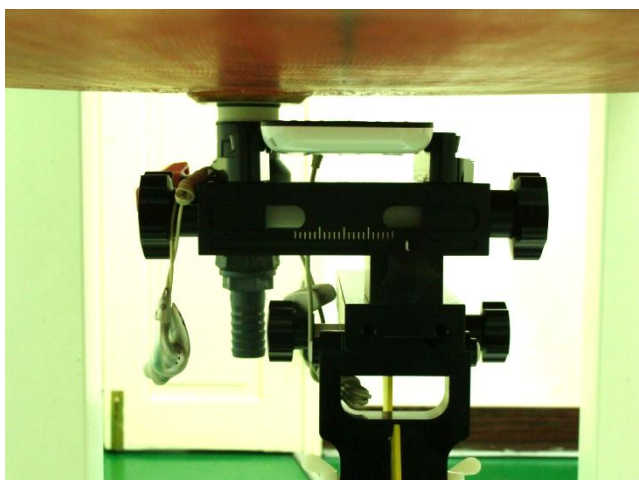
Face of the DUT with Phantom 15 mm Gap
