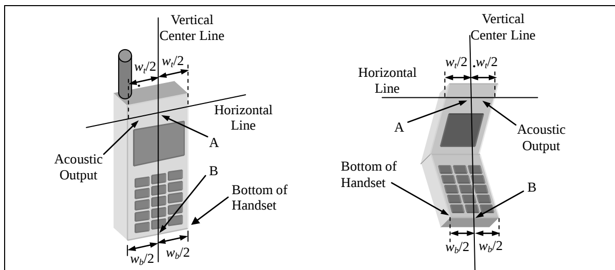
Fig 9.1 Illustration for Handset Vertical and Horizontal Reference Lines
