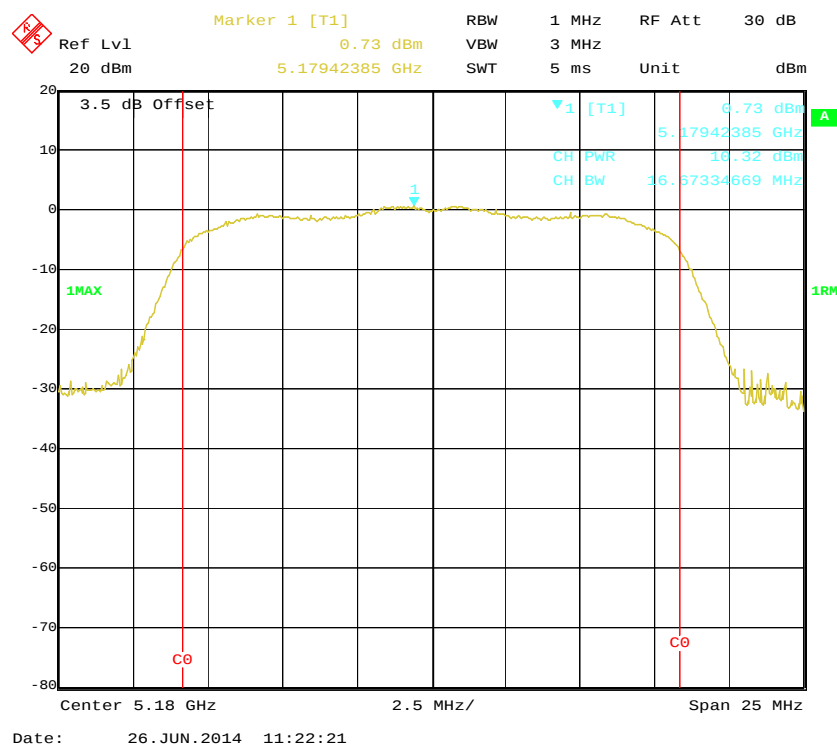
802.11a mode, RF Conducted Output Power, 5180 MHz
