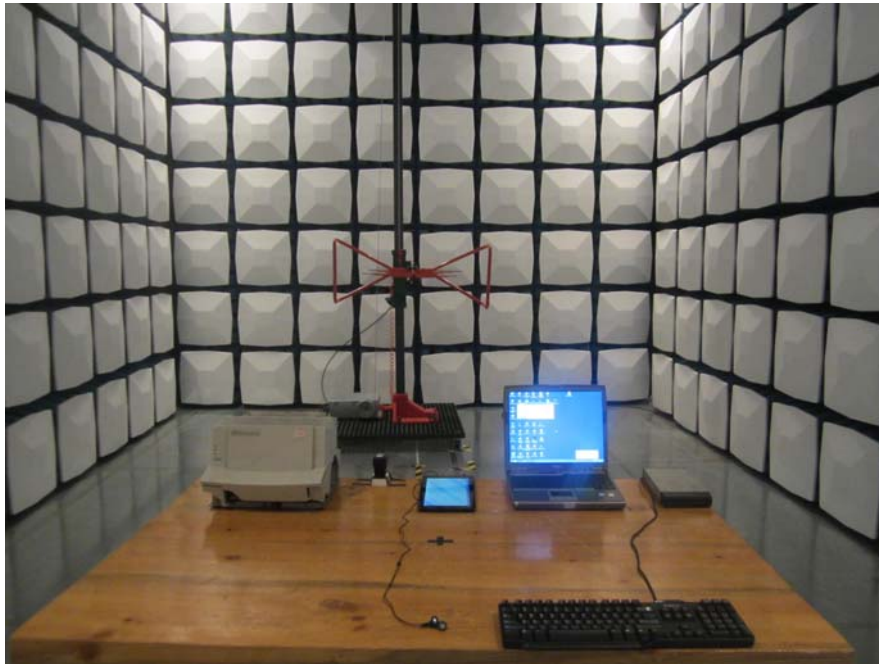
Radiated Emission Below 1GHz -Front View (USB Downloading)
