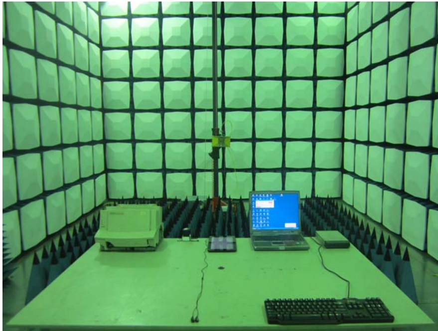
Radiated Emission Above 1GHz -Front View (USB Downloading)
