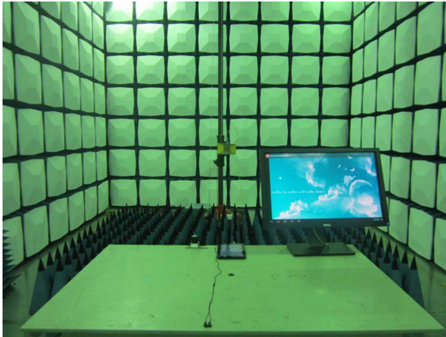
Radiated Emission Above 1GHz -Front View (HDMI Playing)
