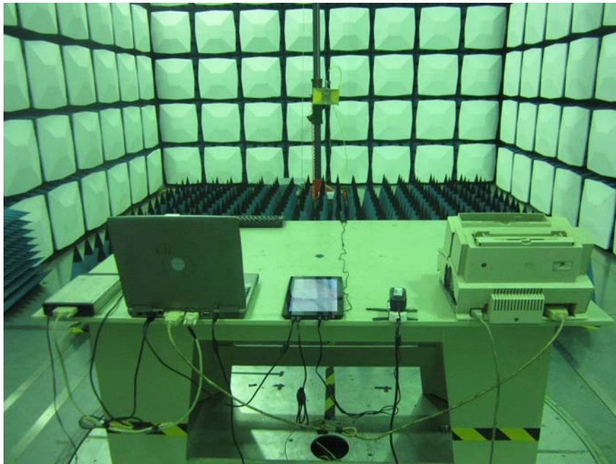
Radiated Emission Above 1GHz - Rear View (USB Downloading)
