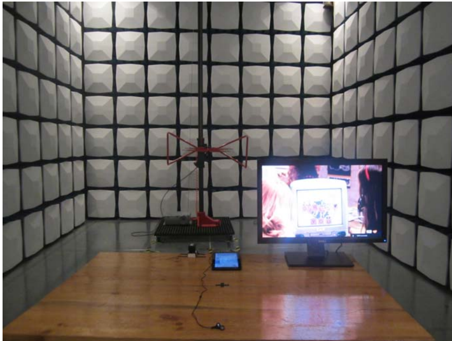
Radiated Emission Below 1GHz -Front View (HDMI Playing)
