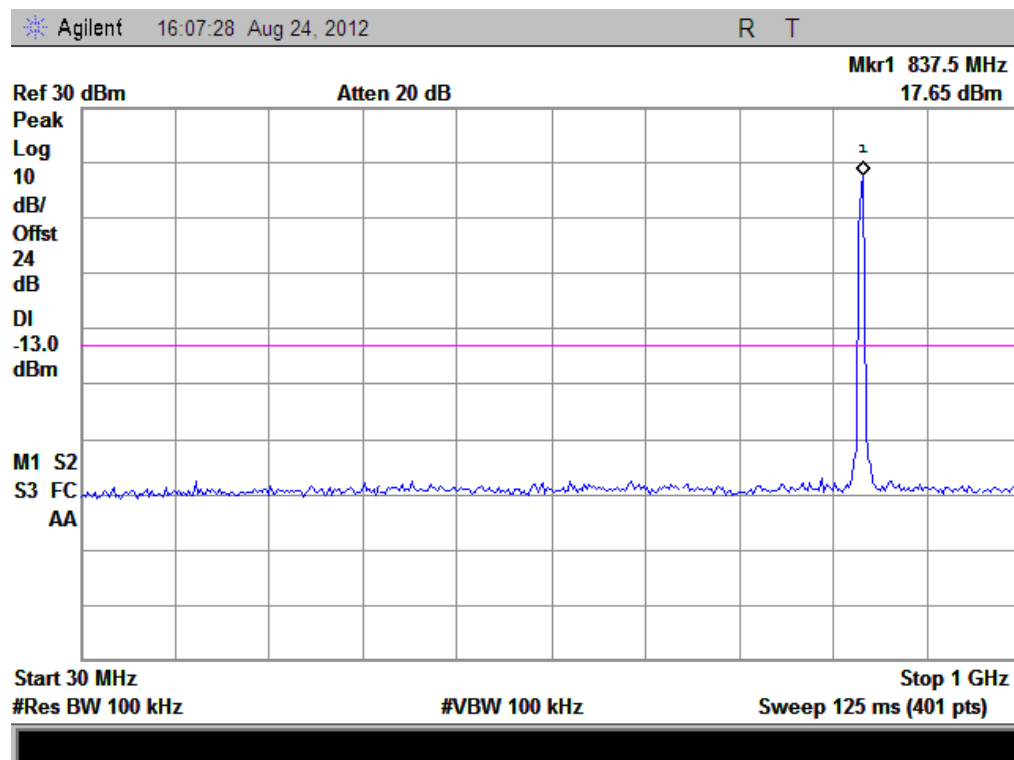
(Plot C2: HSDPA 850MHz Channel = 4175, 30MHz to 1GHz)
