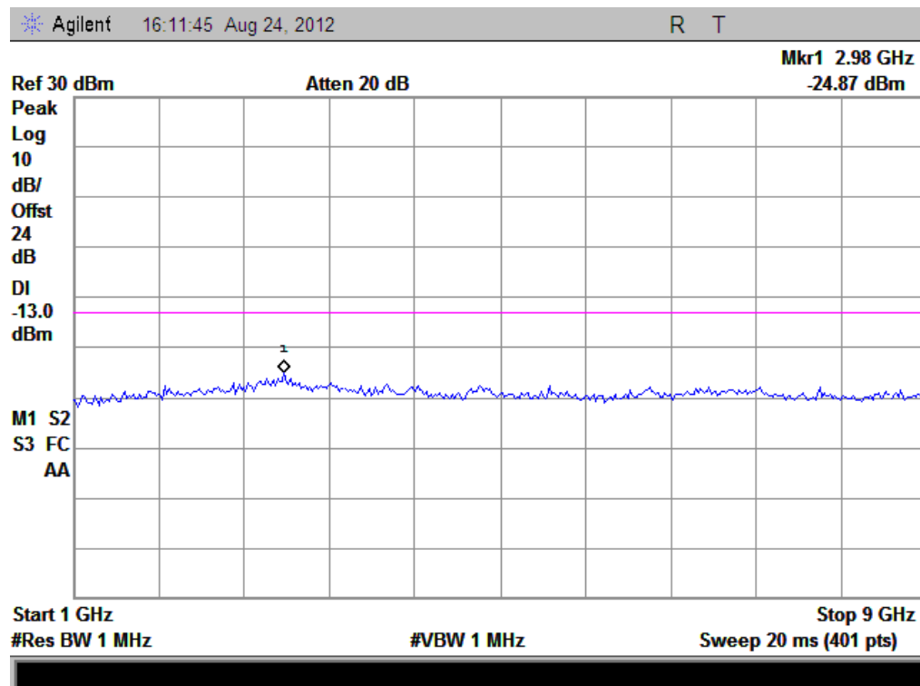
(Plot C2.1: HSDPA 850MHz Channel = 4175, 1GHz to 9GHz)
