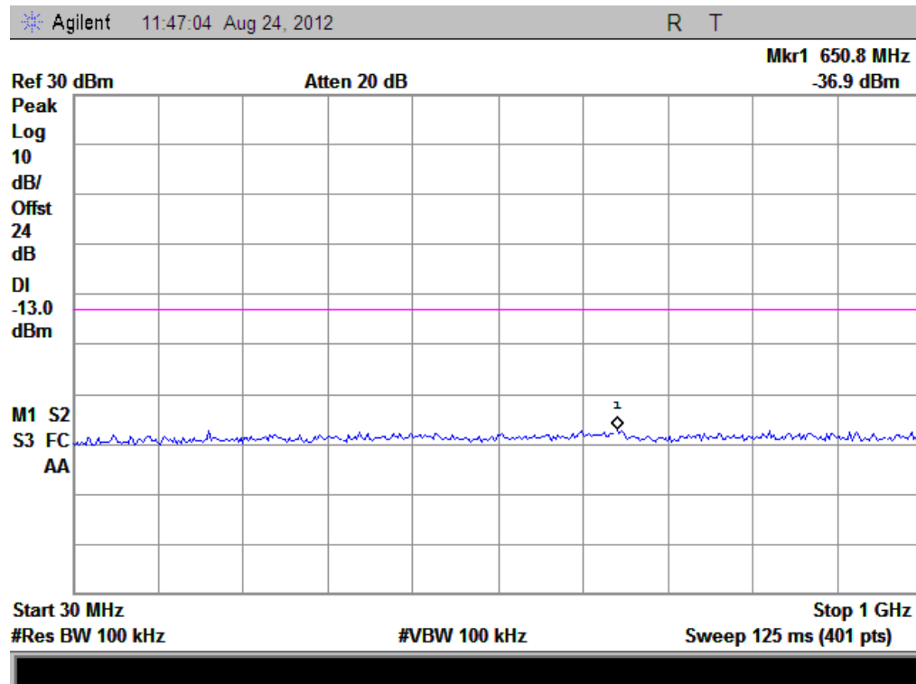
(Plot B3: WCDMA1900MHz Channel = 9538, 30MHz to 1GHz)
