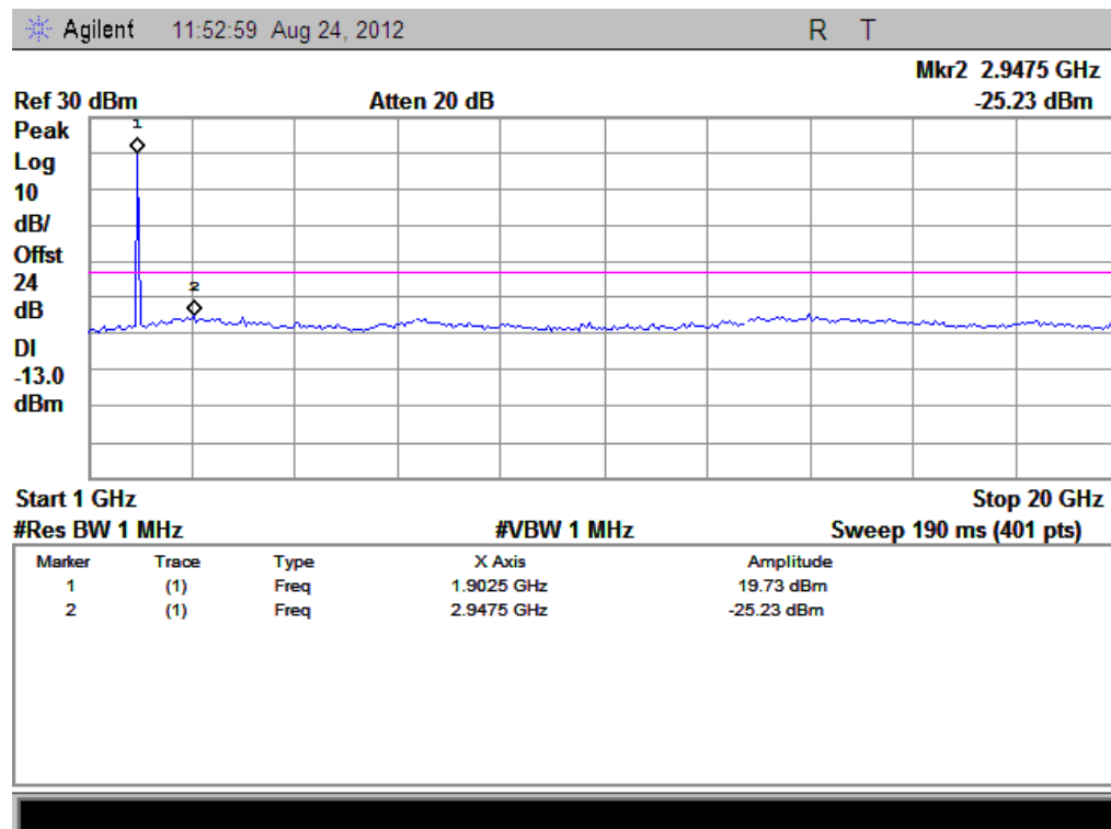
(Plot B3.1: WCDMA1900MHz Channel = 9538 1GHz to 20GHz)
