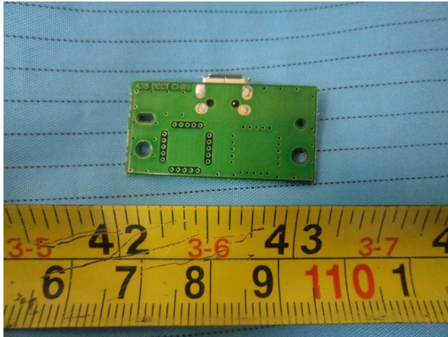
EUT – Charging Base Board Bottom View
