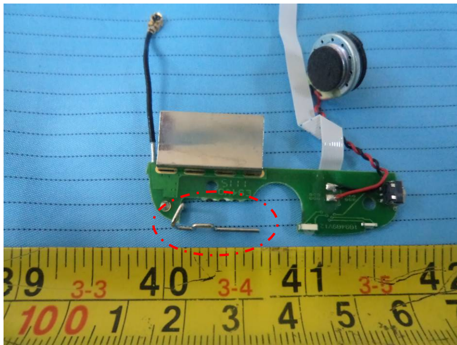
EUT – DECT Antenna View
