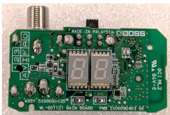
PCB backside
