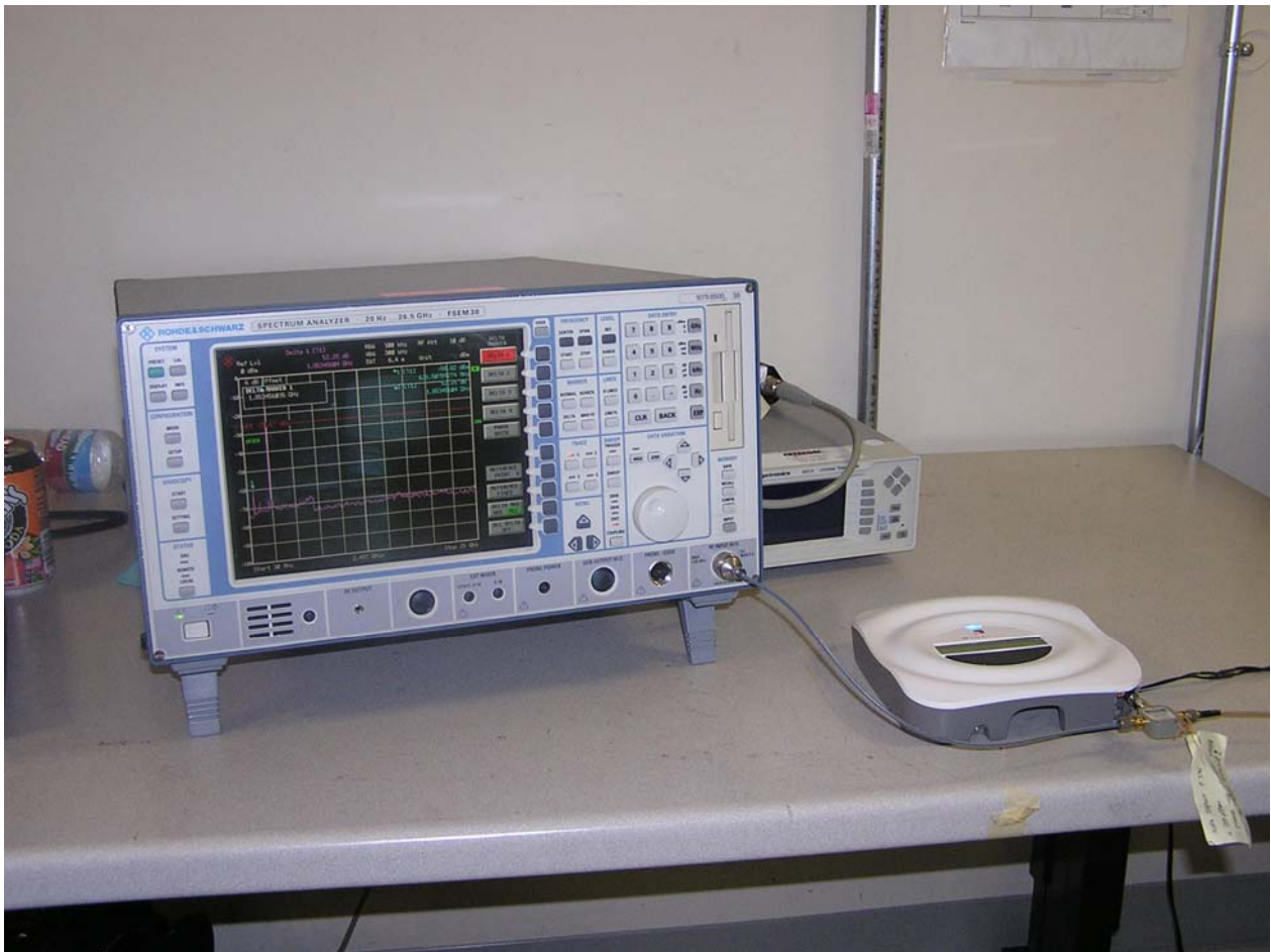
ANTENNA PORT CONDUCTED MEASUREMENT
