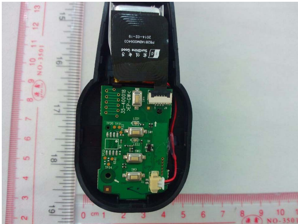
EUT INTERNAL RF BOARD 1
