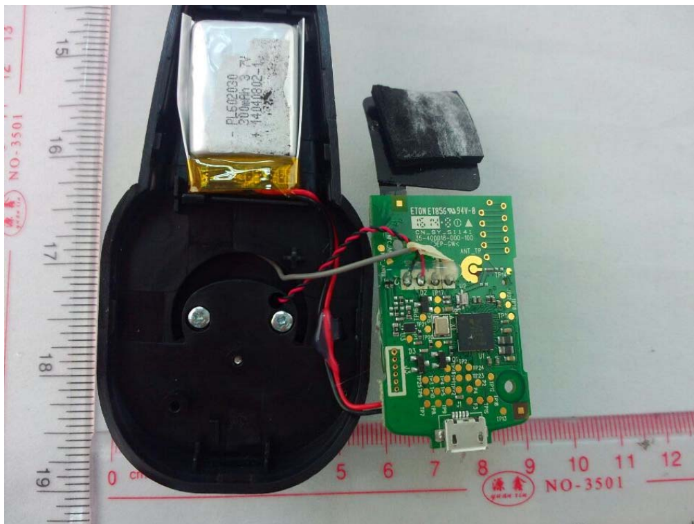
EUT INTERNAL RF BOARD 2
