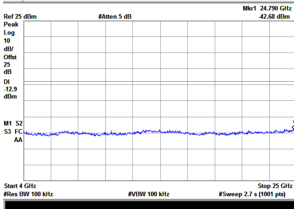
(Plot E.2: Channel = 39, 4GHz to 25GHz)
