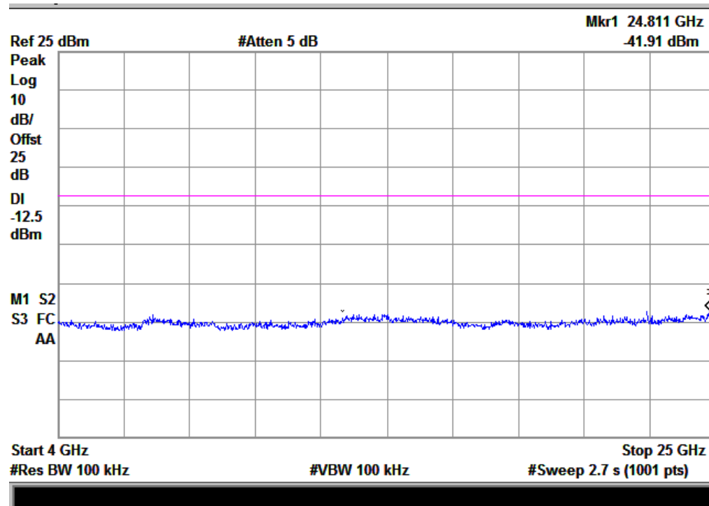
(Plot F.2: Channel = 78, 4GHz to 25GHz)
