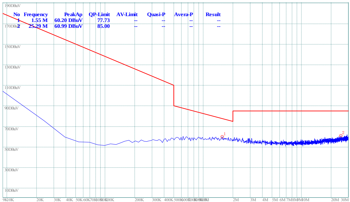
(Plot C.0: 9kHz to 30MHz)
