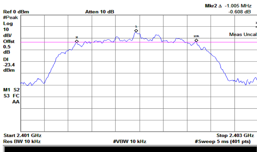
(Plot G: Channel = 2402)
