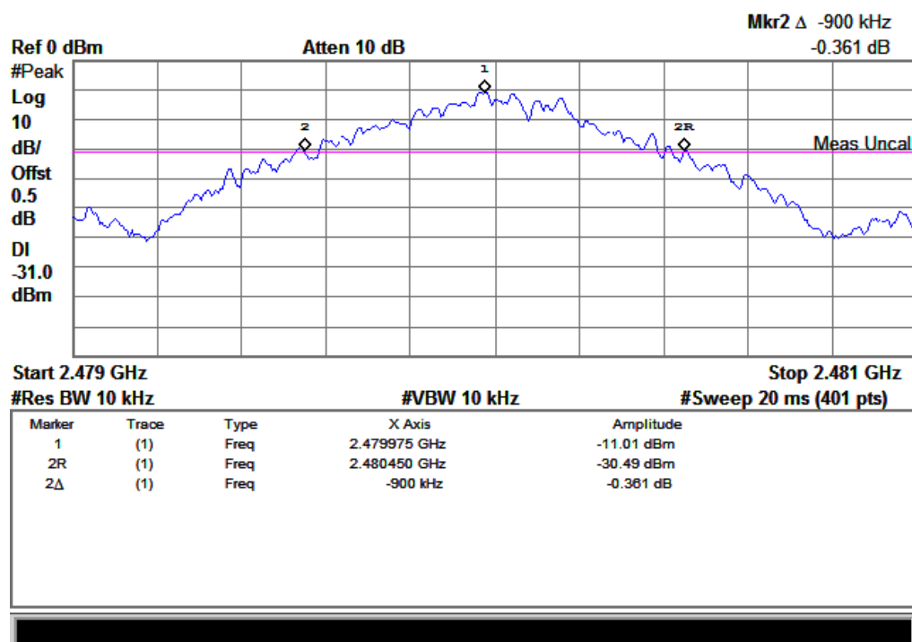
(Plot C: Channel = 2480)
