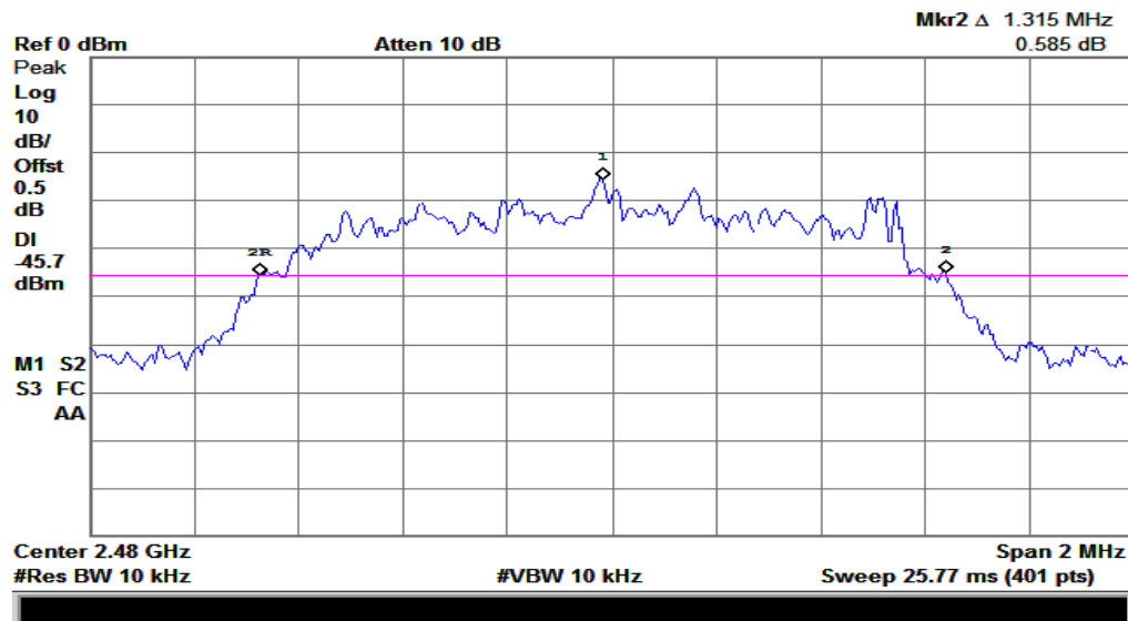
(Plot F: Channel = 2480)
