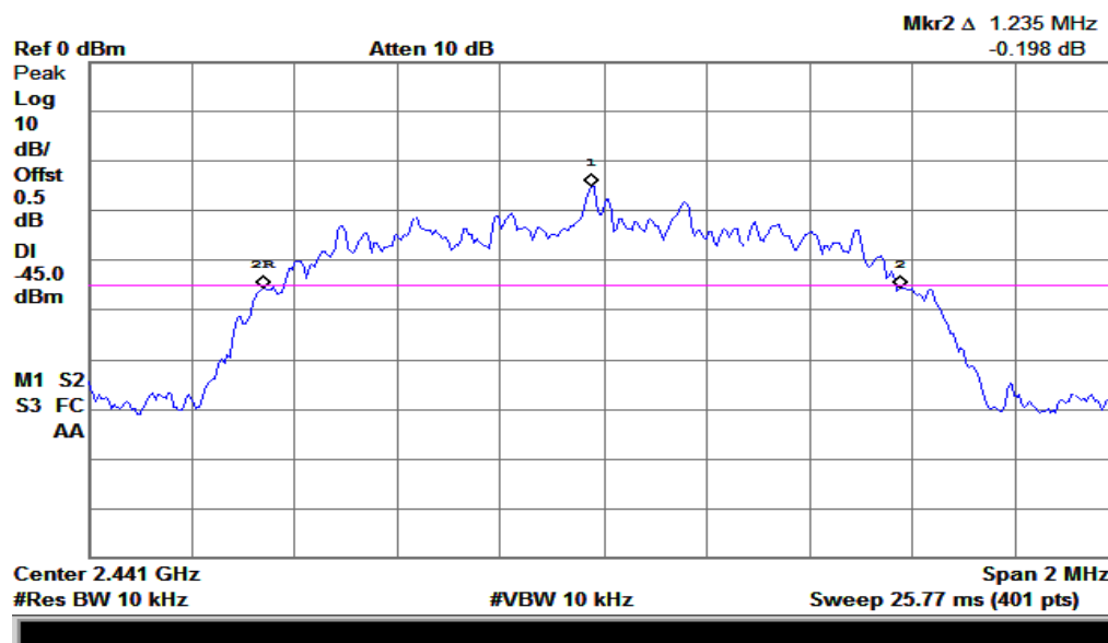
(Plot E: Channel = 2441)
