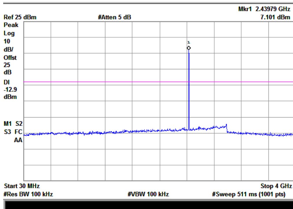
(Plot E.1: Channel = 39, 30MHz to 4GHz)
