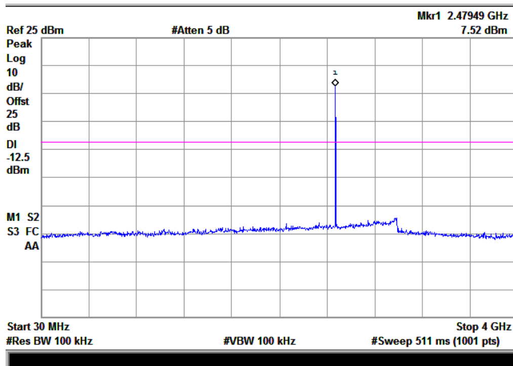
(Plot F.1: Channel = 78, 30MHz to 4GHz)
