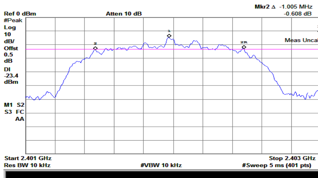
(Plot D: Channel = 2402)
