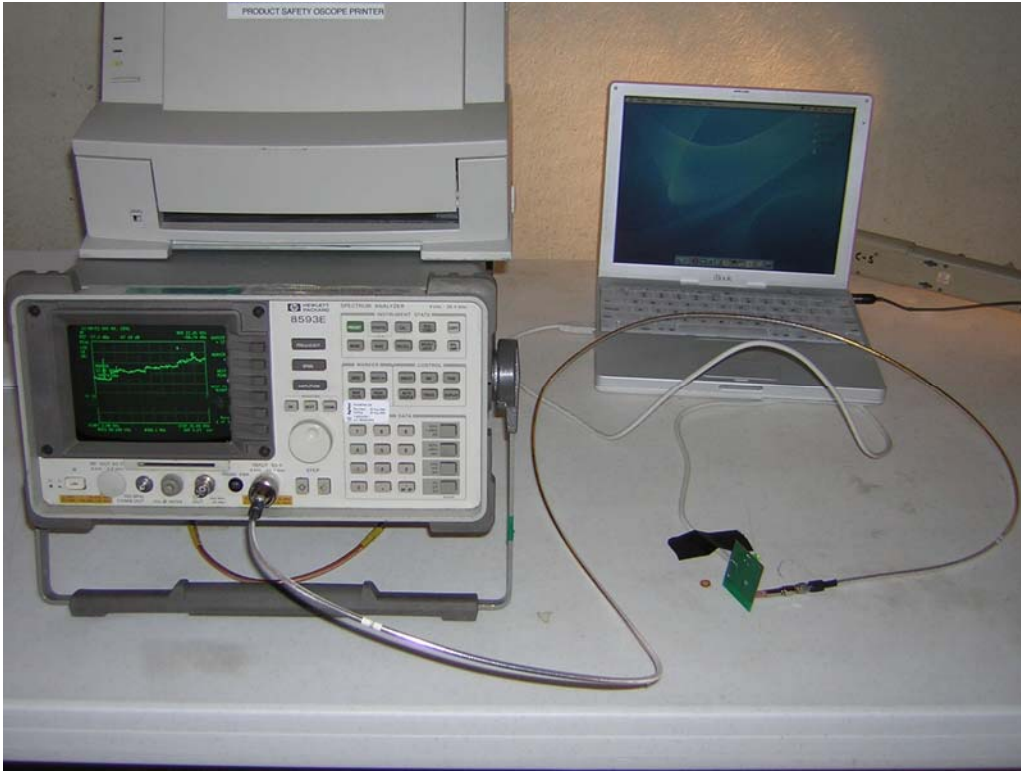
Conducted Antenna Port Measurements
