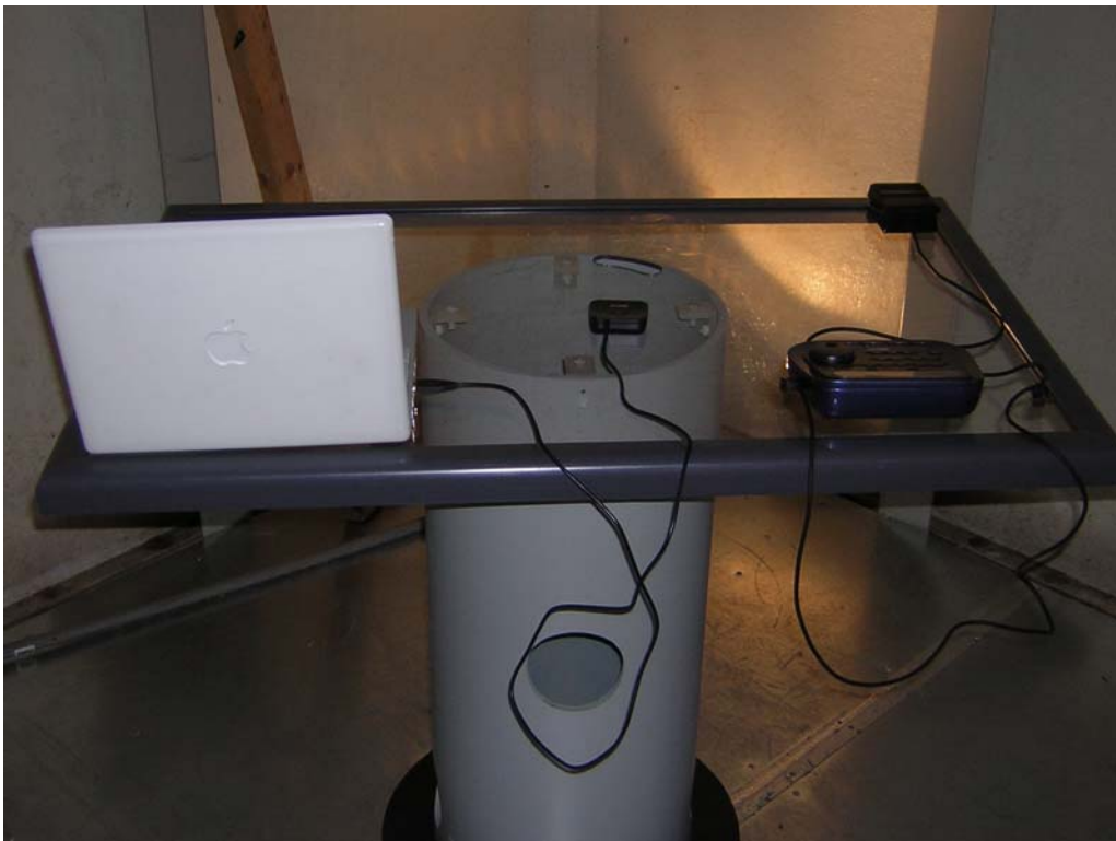
Radiated Emissions
