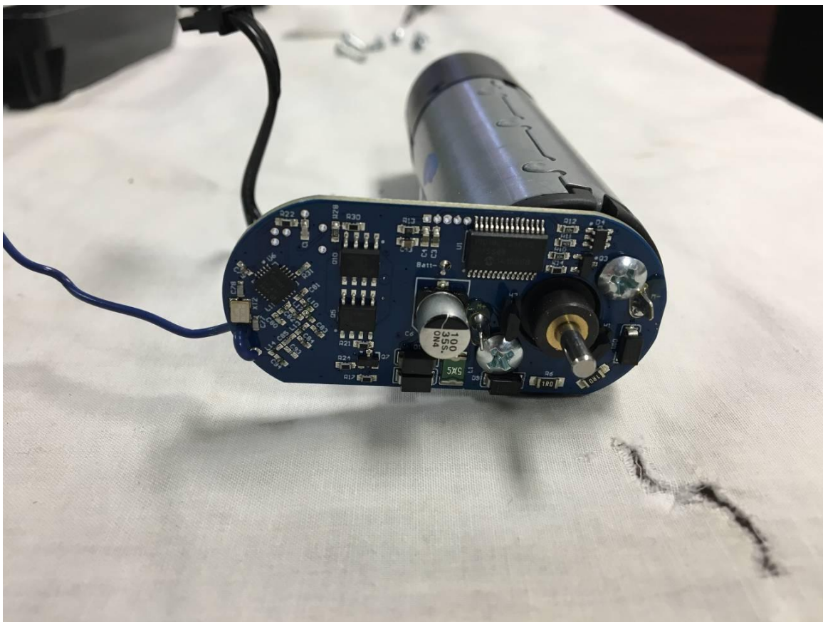
Figure 10. PCB with Radio Circuits
