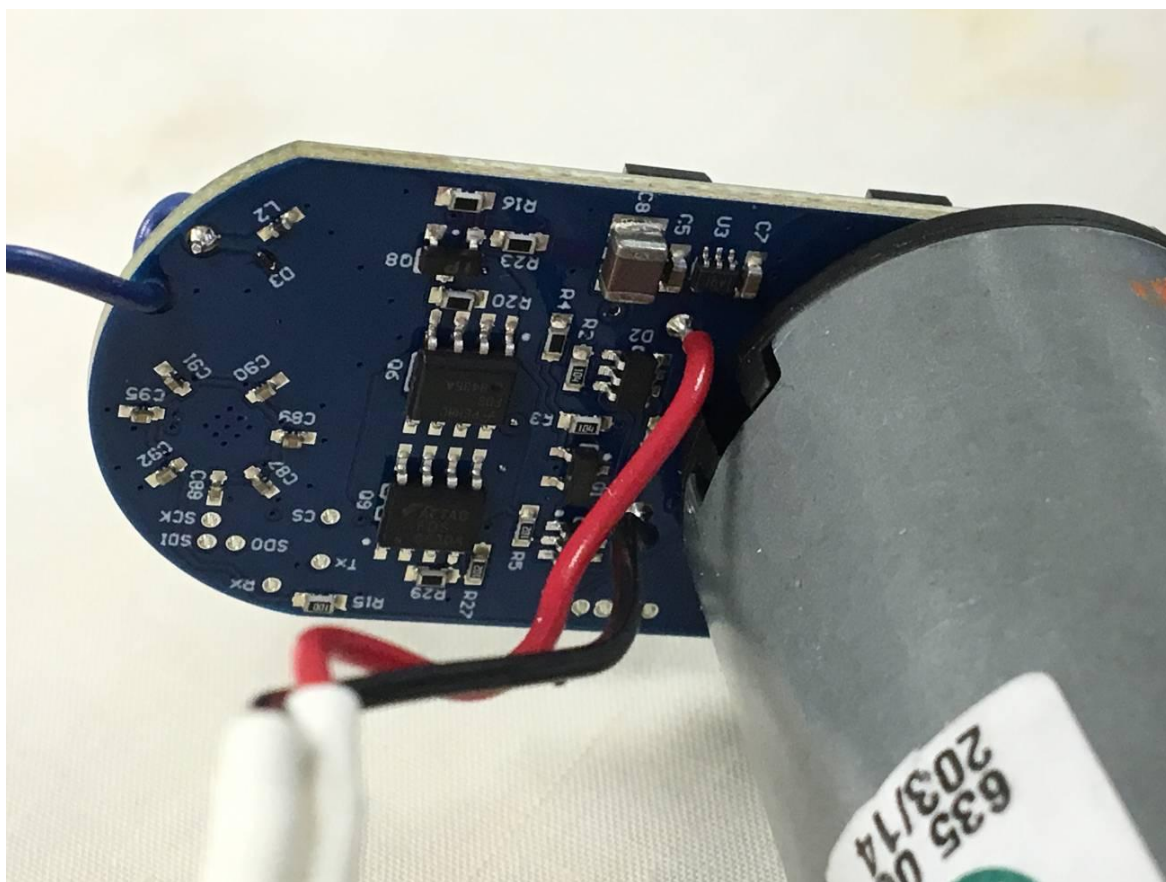
Figure 11. PCB Back Side
