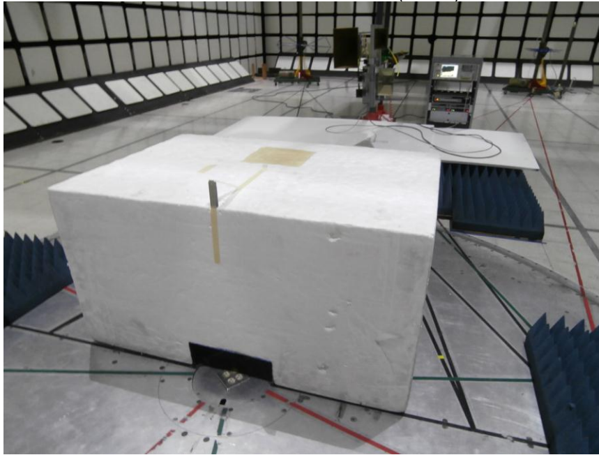
RADIATED EMISSIONS ABOVE 1GHz30 MHz (BACK)
