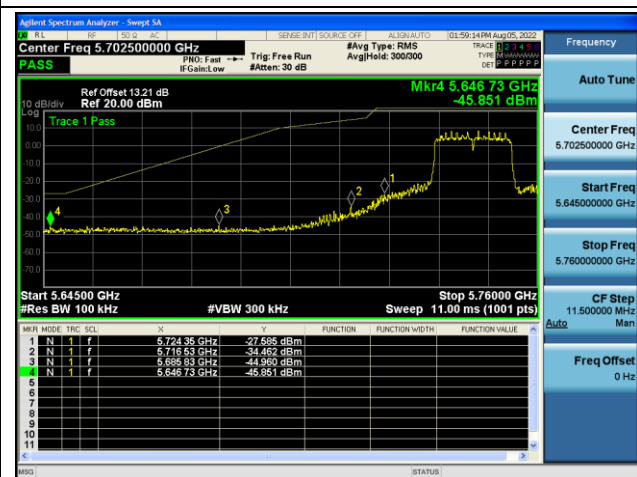
Band edge-Left
