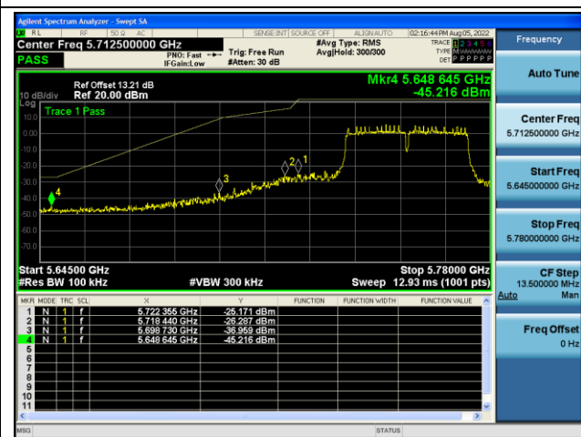
Band edge-Left
