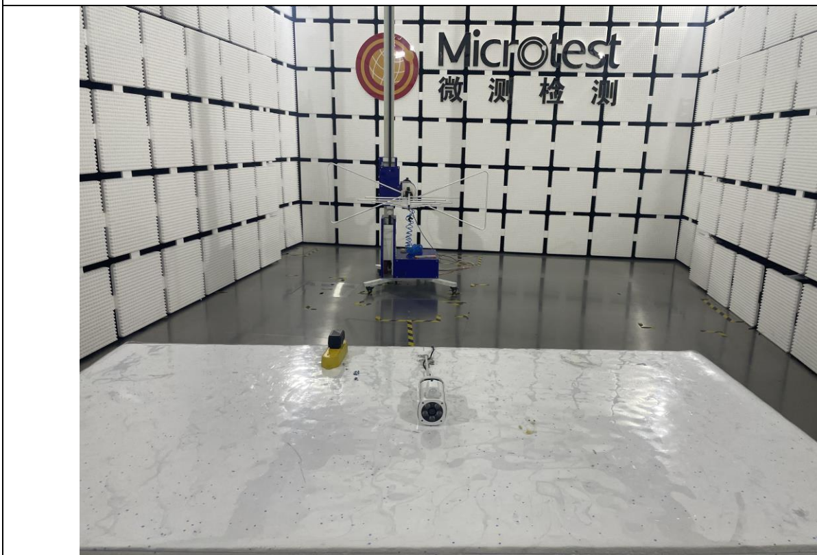
Radiated emission
