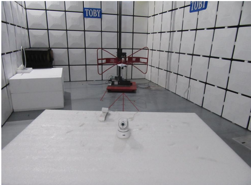
Test Setup
