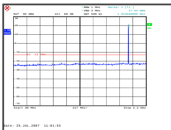
Figure 45: Spurious Emissions - Uplink GSM High Channel – 30 MHz to 2.2 GHz
