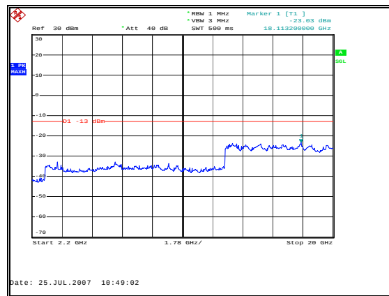
Figure 42: Spurious Emissions - Uplink GSM Low Channel – 2.2 GHz to 20 GHz
