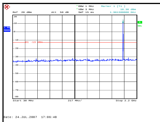
Figure 71: Spurious Emissions - Downlink GSM Mid Channel – 30 MHz to 2.2 GHz
