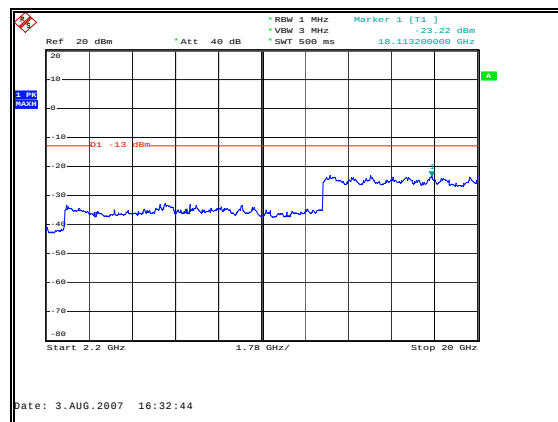
Figure 51: Spurious Emissions - Downlink CDMA Mid Channel – 2.2 GHz to 20 GHz
