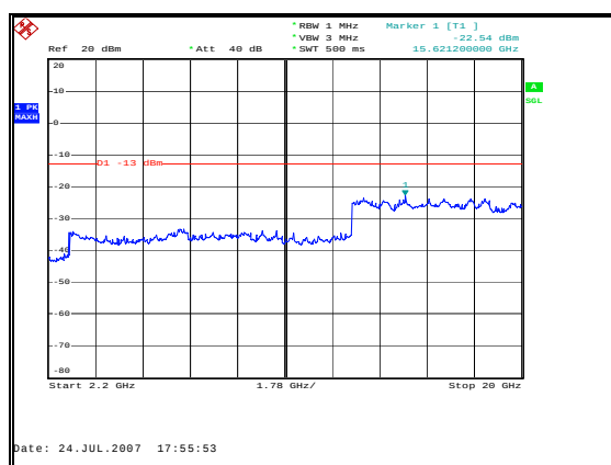
Figure 65: Spurious Emissions - Downlink CW Low Channel – Inter-modulation-2 GHz to 20 GHz
