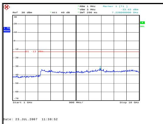
Figure 46: Spurious Emissions - Uplink GSM High Channel – 1 to 10 GHz
