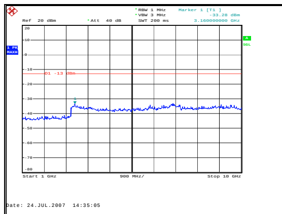
Figure 62: Spurious Emissions - Downlink TDMA High Channel – Inter-modulation - 1 to 10 GHz
