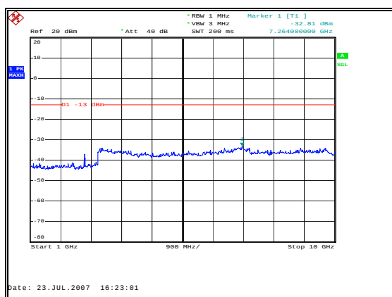
Figure 49: Spurious Emissions - Downlink CDMA Low Channel – Inter-modulation - 1 to 10 GHz
