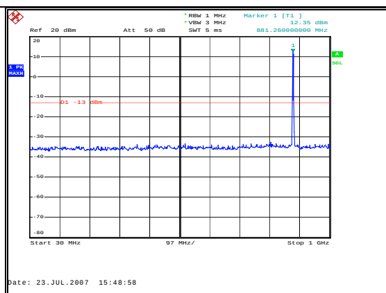
Figure 50: Spurious Emissions - Downlink CDMA Mid Channel – 30 MHz to 1 GHz
