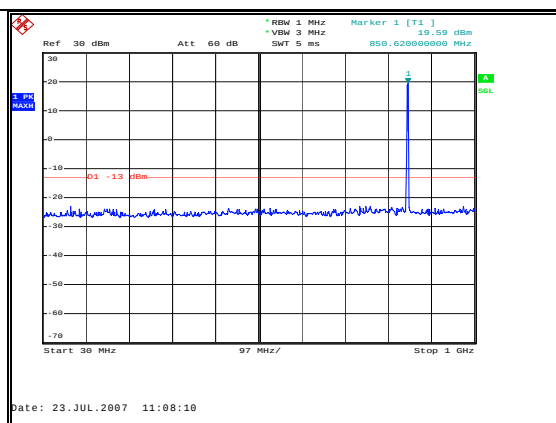
Figure 33: Spurious Emissions - Uplink TDMA High Channel – Inter-modulation - 30 MHz to 1 GHz
