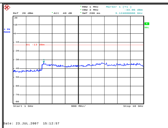
Figure 72: Spurious Emissions - Downlink GSM Mid Channel – 1 to 10 GHz
