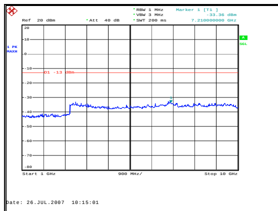
Figure 54: Spurious Emissions - Downlink CDMA High Channel – Inter-modulation - 1 to 10 GHz
