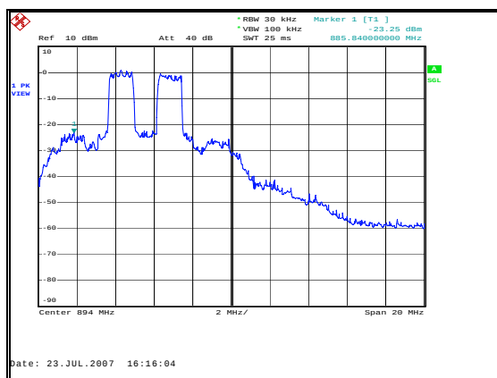
Figure 52: Spurious Emissions - Downlink CDMA High Channel – Inter-modulation In Band
