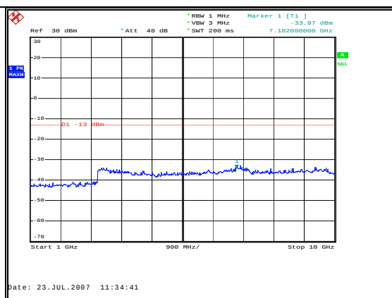
Figure 44: Spurious Emissions - Uplink GSM Mid Channel – 1 to 10 GHz
