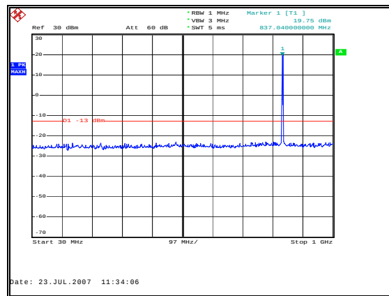
Figure 43: Spurious Emissions - Uplink GSM Mid Channel – 30 MHz to 1 GHz
