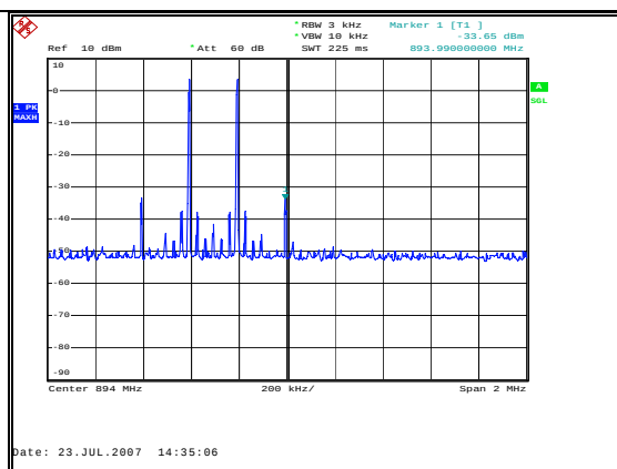
Figure 66: Spurious Emissions - Downlink CW High Channel – Inter-modulation In Band
