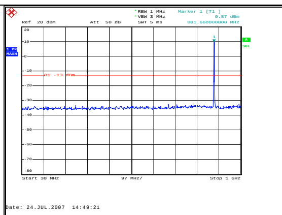
Figure 58: Spurious Emissions - Downlink TDMA Mid Channel – 30 MHz to 1 GHz
