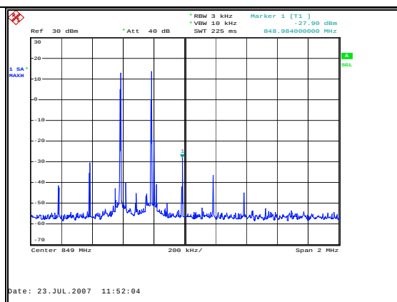
Figure 38: Spurious Emissions - Uplink CW High Channel – Inter-modulation In Band
