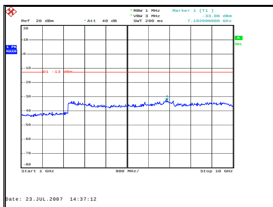
Figure 68: Spurious Emissions - Downlink CW High Channel – Inter-modulation - 1 to 10 GHz
