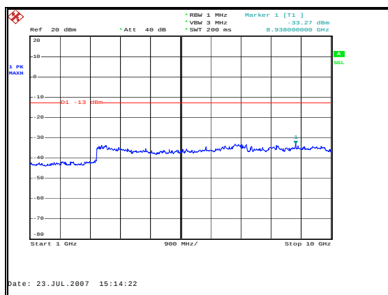
Figure 74: Spurious Emissions - Downlink GSM High Channel – 1 to 10 GHz
