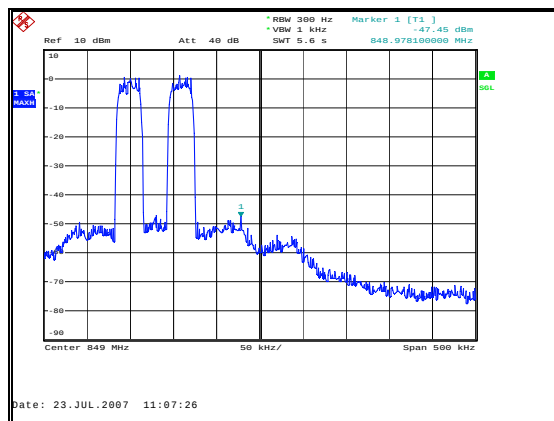
Figure 32: Spurious Emissions - Uplink TDMA High Channel – Inter-modulation In Band
