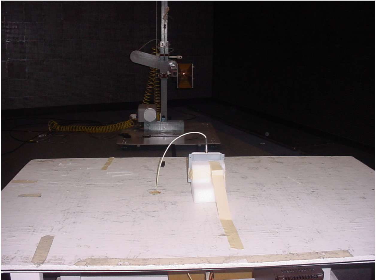
Figure 3: Radiated Emissions Test Setup
