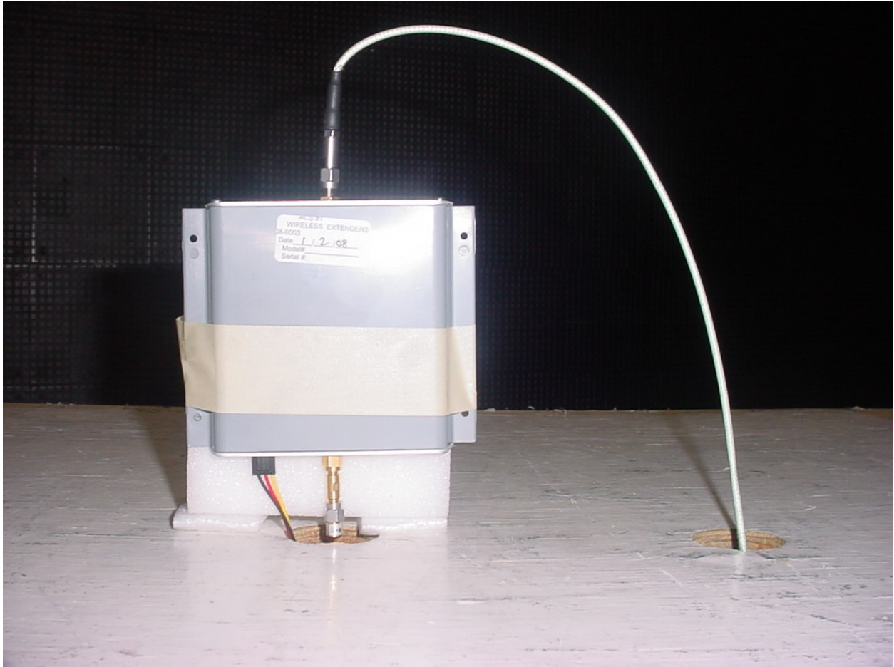
Figure 2: Radiated Emissions Test Setup
