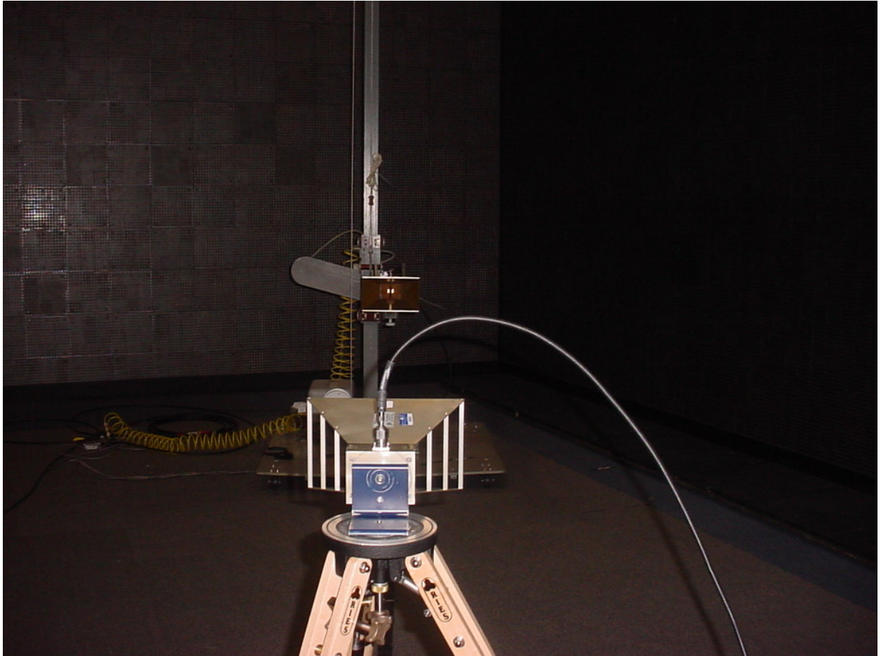
Figure 4: Radiated Emissions Test Setup
