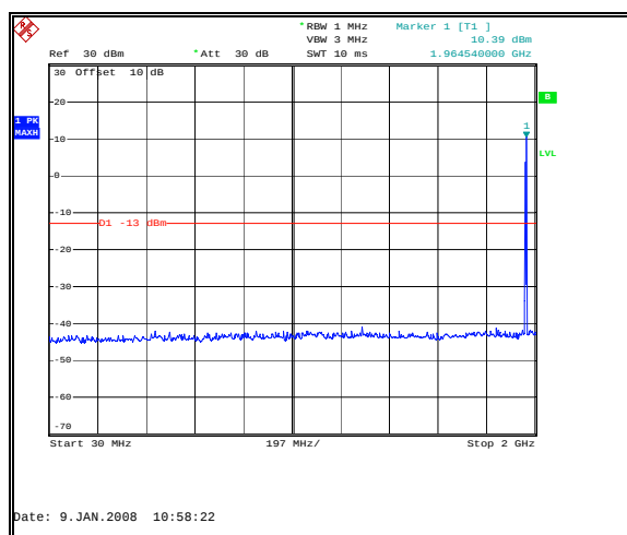
Figure 54: Spurious Emissions - Downlink TDMA Mid Channel – 30 MHz to 2 GHz
