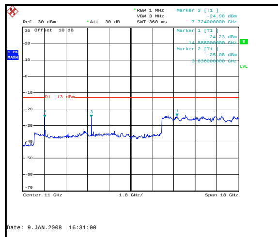
Figure 61: Spurious Emissions - Downlink GSM Low Channel – 2 GHz to 20 GHz
