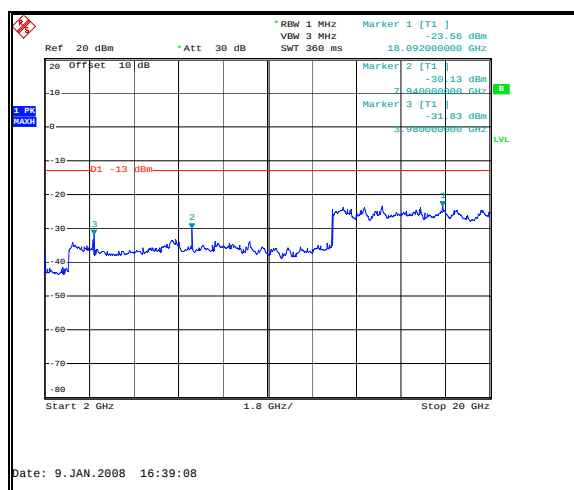
Figure 66: Spurious Emissions - Downlink GSM High Channel – 2 GHz to 20 GHz
