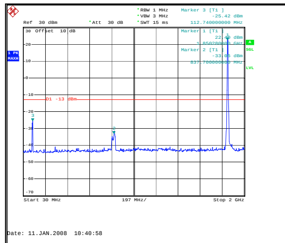
Figure 20: Spurious Emissions - Uplink CDMA Low Channel – Inter-modulation-30 MHz to 2 GHz
