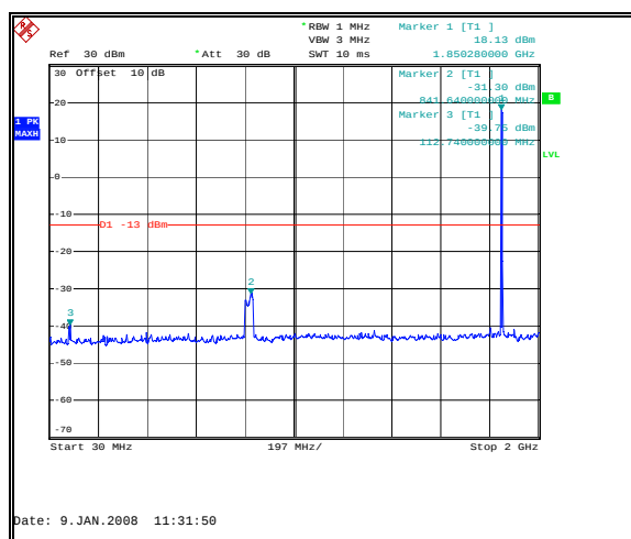
Figure 33: Spurious Emissions - Uplink TDMA High Channel – Inter-modulation-30 MHz to 2 GHz
