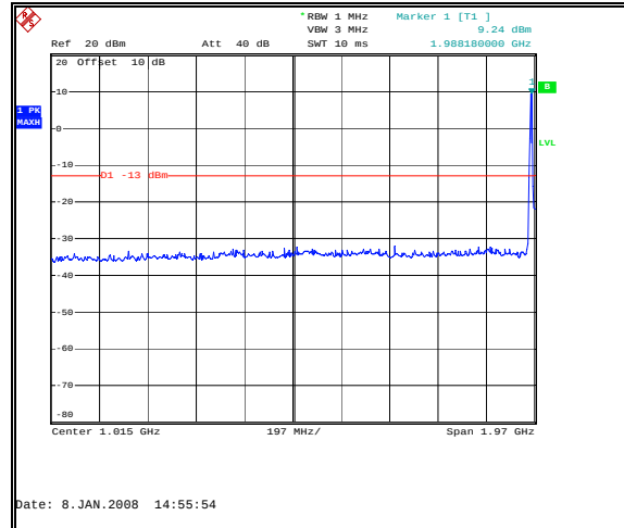
Figure 49: Spurious Emissions-Downlink CDMA High Channel-Inter-modulation-30MHz to 2GHz
