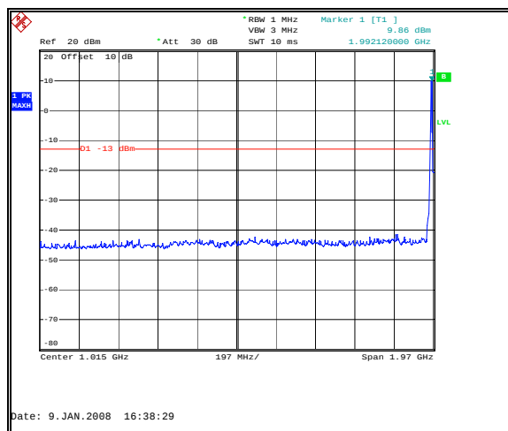
Figure 65: Spurious Emissions - Downlink GSM High Channel – 30 MHz to 2 GHz
