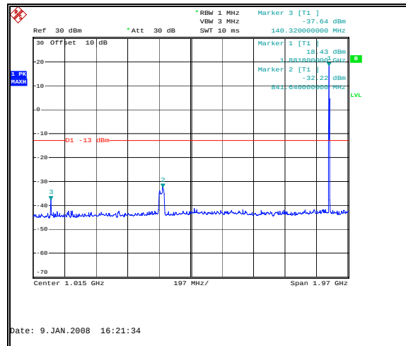
Figure 38: Spurious Emissions - Uplink GSM Mid Channel – 30 MHz to 2 GHz
