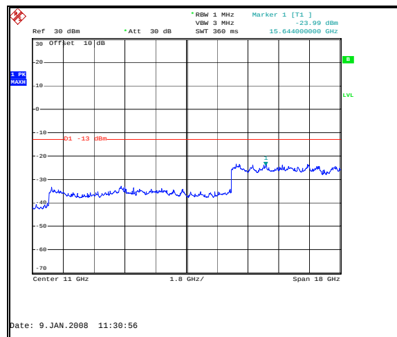
Figure 29: Spurious Emissions - Uplink TDMA Low Channel – Inter-modulation-2 GHz to 20 GHz
