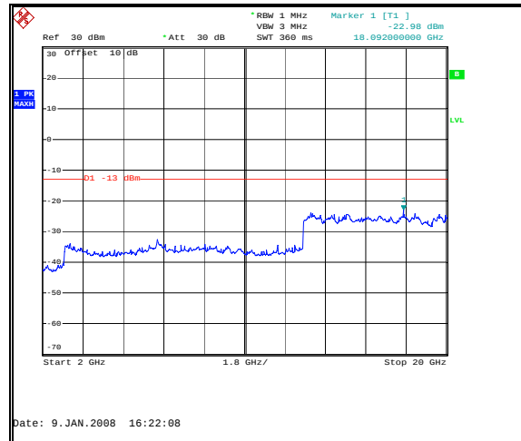
Figure 39: Spurious Emissions - Uplink GSM Mid Channel – 2 GHz to 20 GHz
