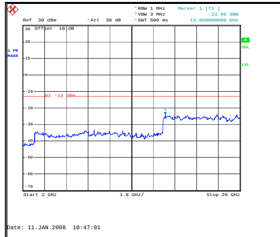
Figure 23: Spurious Emissions - Uplink CDMA Mid Channel – 2 GHz to 20 GHz
