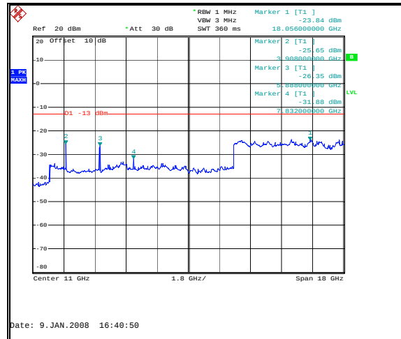
Figure 63: Spurious Emissions - Downlink GSM Mid Channel – 2 GHz to 20 GHz
