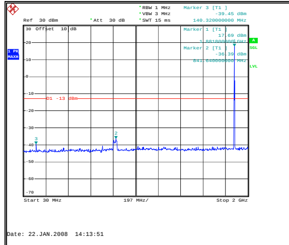
Figure 30: Spurious Emissions - Uplink TDMA Mid Channel – 30 MHz to 2 GHz
