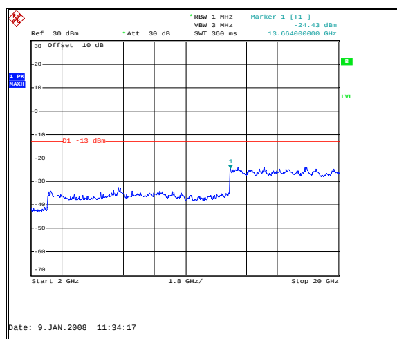
Figure 34: Spurious Emissions - Uplink TDMA High Channel – Inter-modulation-2 GHz to 20 GHz
