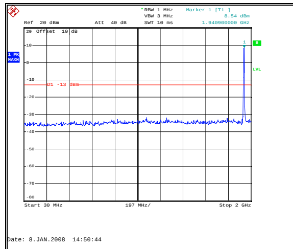
Figure 44: Spurious Emissions-Downlink CDMA Low Channel-Inter-modulation-30MHz to 2GHz
