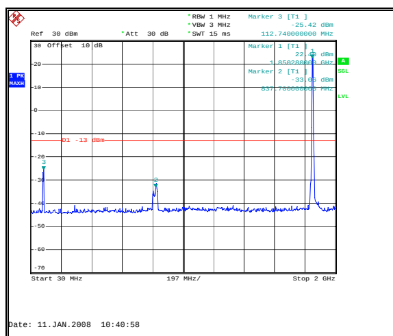
Figure 25: Spurious Emissions - Uplink CDMA High Channel-Inter-modulation-30 MHz to 2 GHz
