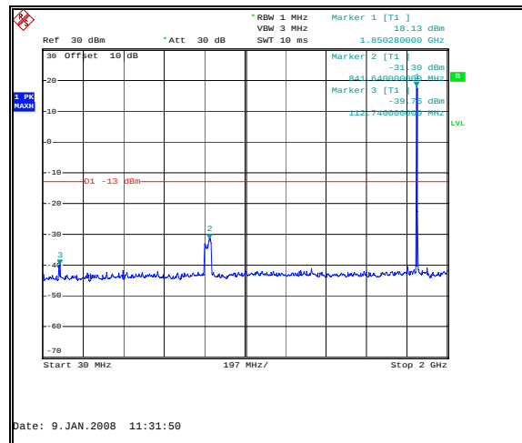
Figure 28: Spurious Emissions - Uplink TDMA Low Channel – Inter-modulation-30 MHz to 2 GHz
