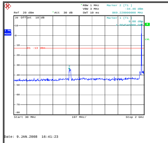
Figure 62: Spurious Emissions - Downlink GSM Mid Channel – 30 MHz to 2 GHz
