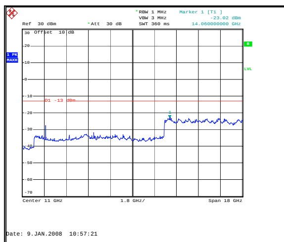
Figure 55: Spurious Emissions - Downlink TDMA Mid Channel – 2 GHz to 20 GHz
