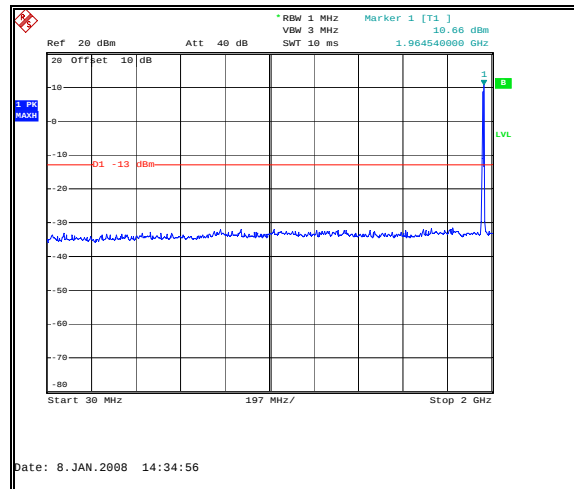
Figure 46: Spurious Emissions - Downlink CDMA Mid Channel – 30 MHz to 2 GHz
