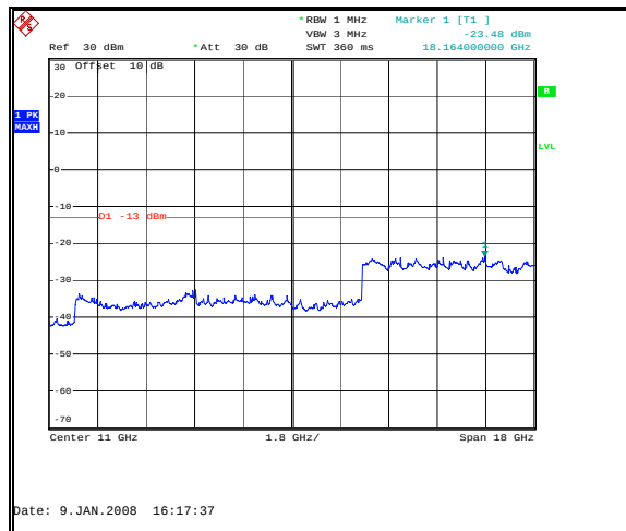
Figure 37: Spurious Emissions - Uplink GSM Low Channel – 2 GHz to 20 GHz
