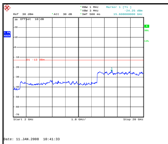
Figure 26: Spurious Emissions - Uplink CDMA High Channel-Inter-modulation-2 GHz to 20 GHz
