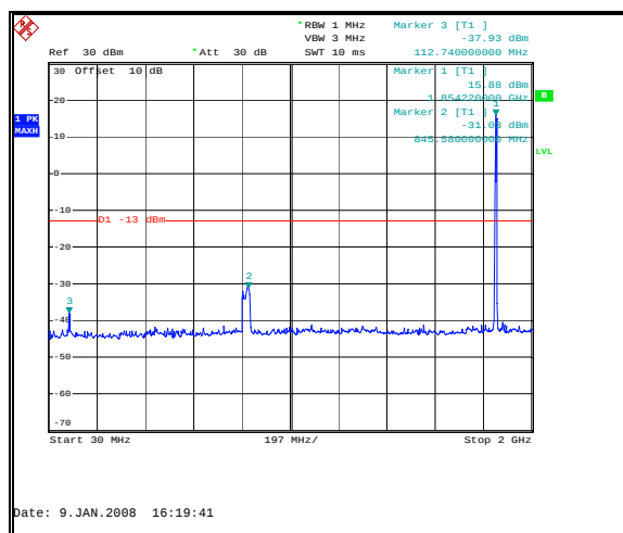
Figure 36: Spurious Emissions - Uplink GSM Low Channel – 30 MHz to 2 GHz
