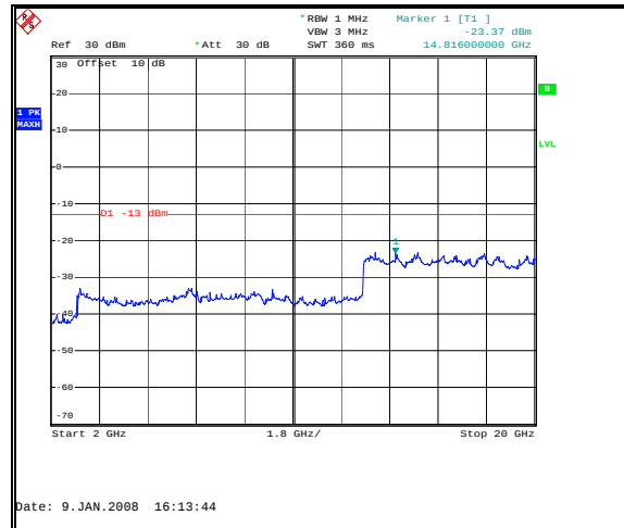
Figure 42: Spurious Emissions - Uplink GSM High Channel – 2 GHz to 20 GHz
