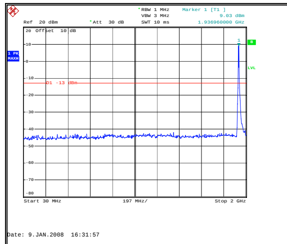
Figure 60: Spurious Emissions - Downlink GSM Low Channel – 30 MHz to 2 GHz
