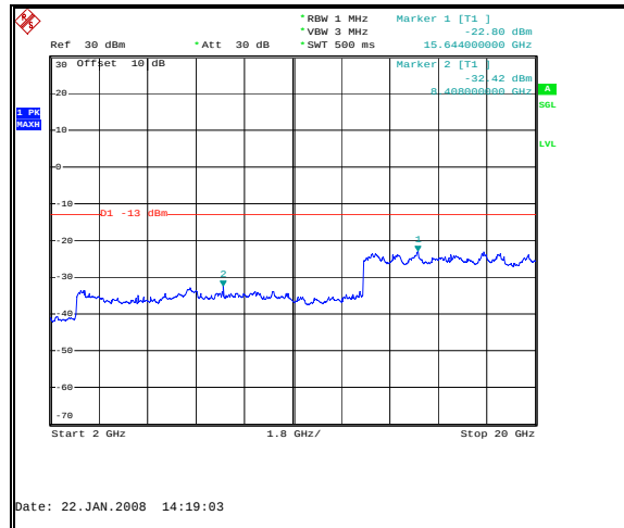
Figure 31: Spurious Emissions - Uplink TDMA Mid Channel – 2 GHz to 20 GHz
