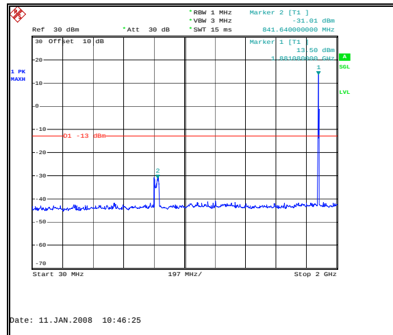
Figure 22: Spurious Emissions - Uplink CDMA Mid Channel – 30 MHz to 2 GHz
