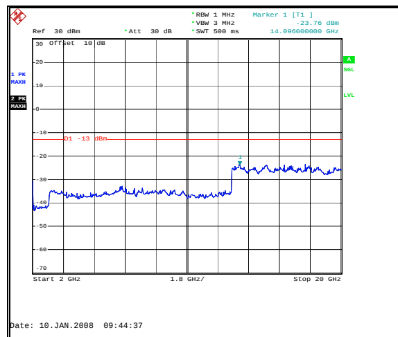
Figure 45: Spurious Emissions-Downlink CDMA Low Channel-Inter-modulation-2 GHz to 20 GHz
