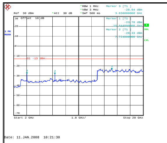
Figure 53: Spurious Emissions-Downlink TDMA Low Channel–Inter-modulation-2GHz to20 GHz
