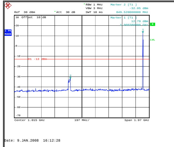
Figure 41: Spurious Emissions - Uplink GSM High Channel – 30 MHz to 2 GHz
