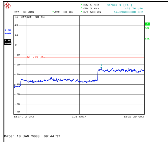
Figure 50: Spurious Emissions-Downlink CDMA High Channel-Inter-modulation-2GHz to 20GHz
