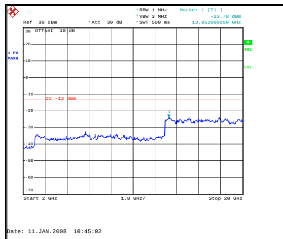
Figure 21: Spurious Emissions - Uplink CDMA Low Channel – Inter-modulation-2 GHz to 20 GHz
