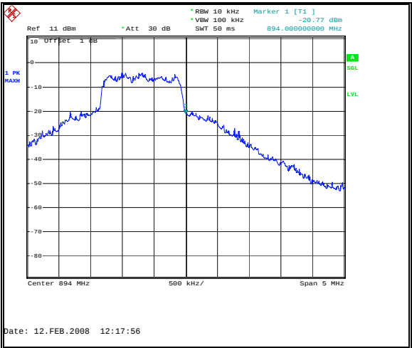
Figure74: Band-Edge Downlink CDMA High Channel
