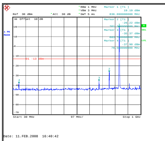
Figure 38: Spurious Emissions - Uplink GSM Mid Channel – 30 MHz to 1 GHz
