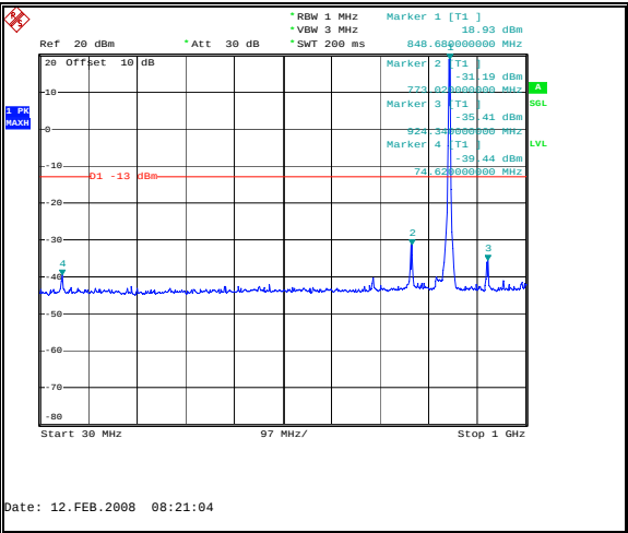
Figure 41: Spurious Emissions - Uplink GSM High Channel – Inter-modulation - 30 MHz to 1 GHz
