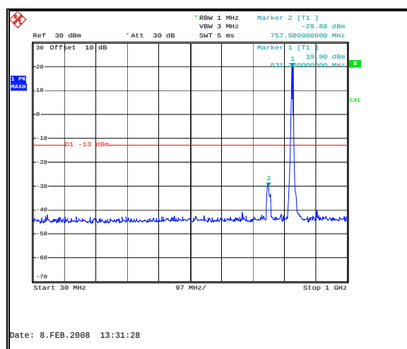
Figure 20: Spurious Emissions - Uplink CDMA Low Channel – Inter-modulation - 30 MHz to 1 GHz
