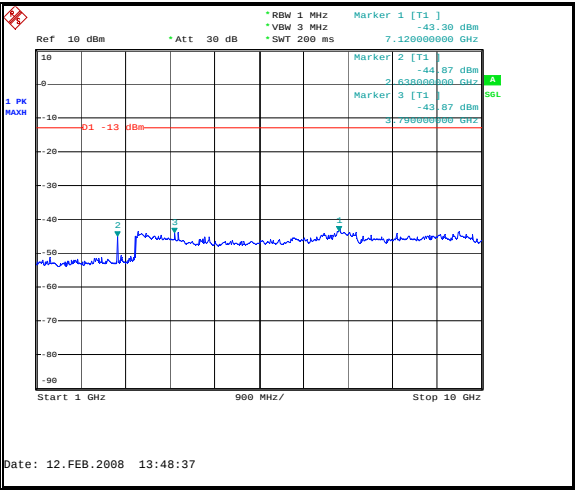
Figure 55: Spurious Emissions - Downlink TDMA Mid Channel – 1 to 10 GHz
