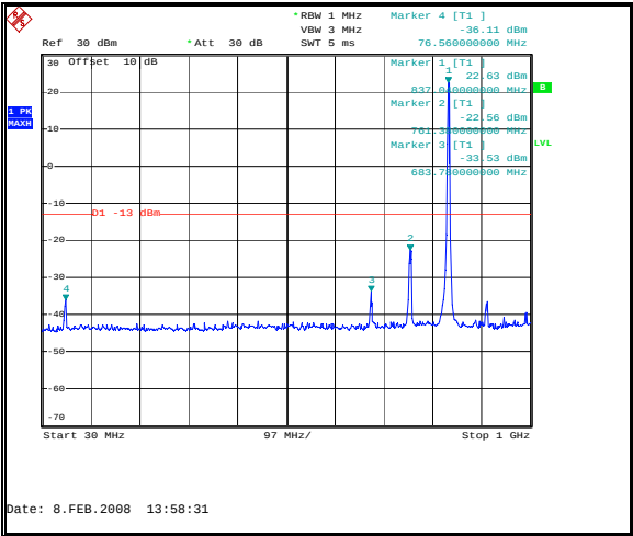
Figure 22: Spurious Emissions - Uplink CDMA Mid Channel – 30 MHz to 1 GHz
