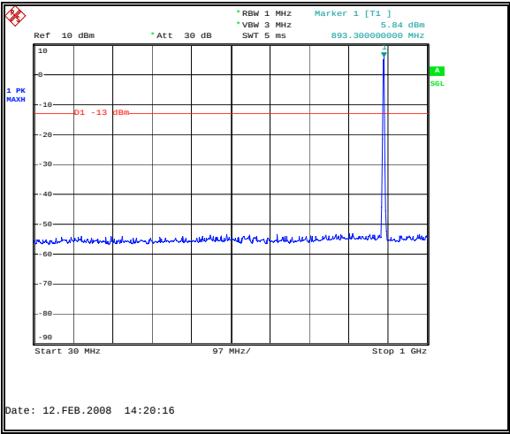
Figure 65: Spurious Emissions - Downlink GSM High Channel – Inter-modulation - 30 MHz to 1 GHz
