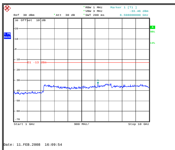
Figure 29: Spurious Emissions - Uplink TDMA Low Channel – Inter-modulation - 1 to 10 GHz
