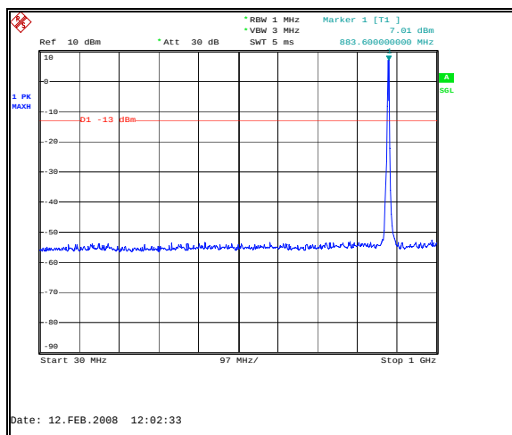
Figure 46: Spurious Emissions - Downlink CDMA Mid Channel – 30 MHz to 1 GHz
