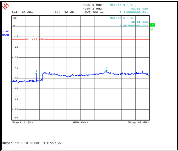
Figure 53: Spurious Emissions - Downlink TDMA Low Channel – Inter-modulation - 1 to 10 GHz
