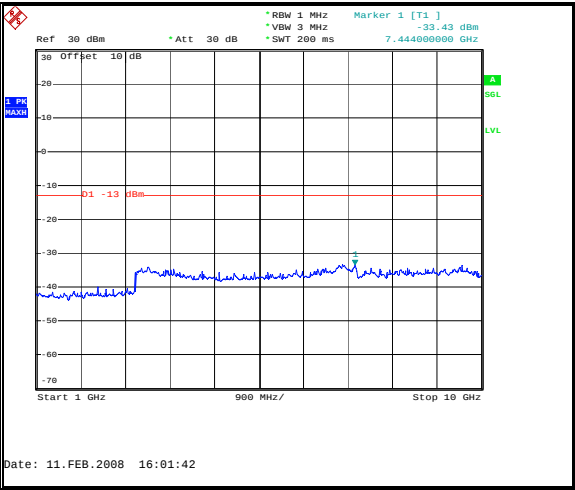
Figure 34: Spurious Emissions - Uplink TDMA High Channel – Inter-modulation - 1 to 10 GHz
