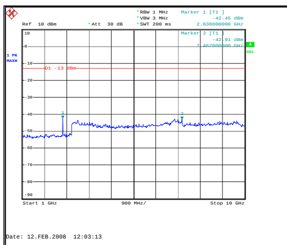
Figure 47: Spurious Emissions - Downlink CDMA Mid Channel – 1 to 10 GHz
