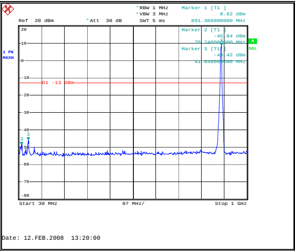
Figure 49: Spurious Emissions - Downlink CDMA High Channel –Inter-modulation-30MHz to 1GHz
