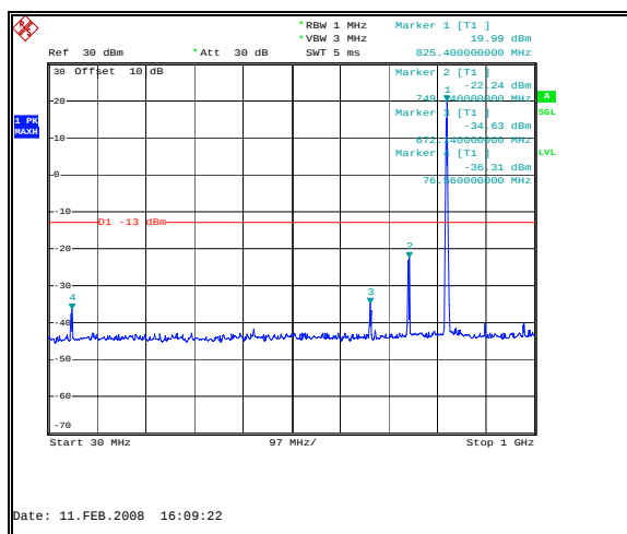
Figure 28: Spurious Emissions - Uplink TDMA Low Channel – Inter-modulation - 30 MHz to 1 GHz
