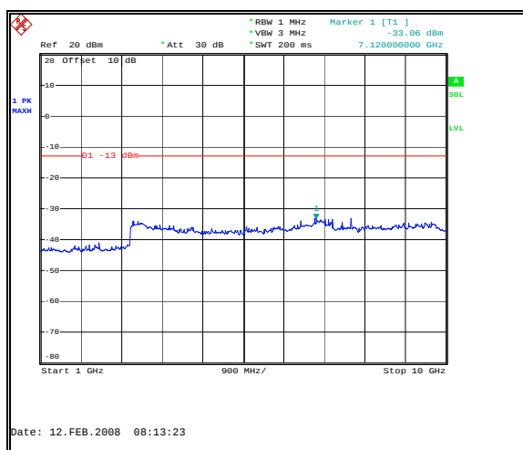
Figure 37: Spurious Emissions - Uplink GSM Low Channel – Inter-modulation - 1 to 10 GHz
