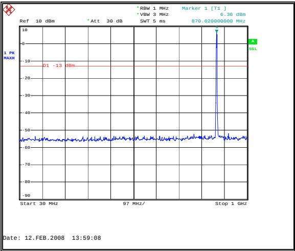
Figure 52: Spurious Emissions - Downlink TDMA Low Channel – Inter-modulation-30MHz to 1GHz
