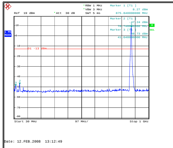
Figure 44: Spurious Emissions - Downlink CDMA Low Channel – Inter-modulation-30MHz to 1GHz
