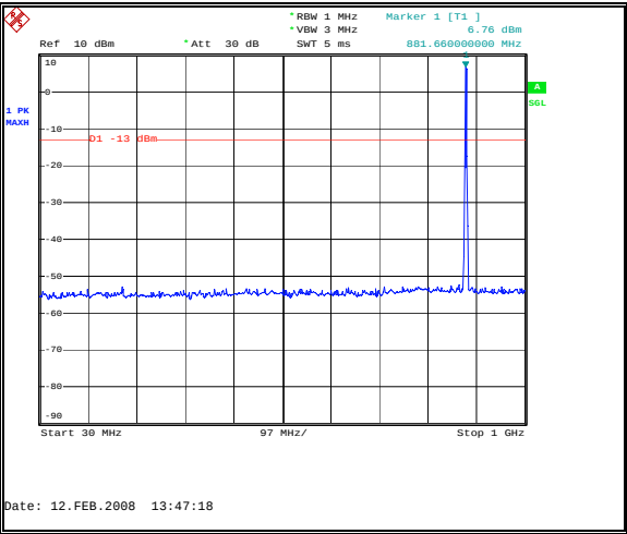
Figure 54: Spurious Emissions - Downlink TDMA Mid Channel – 30 MHz to 1 GHz
