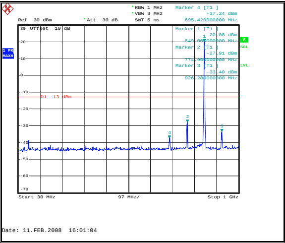
Figure 33: Spurious Emissions - Uplink TDMA High Channel – Inter-modulation - 30 MHz to 1 GHz
