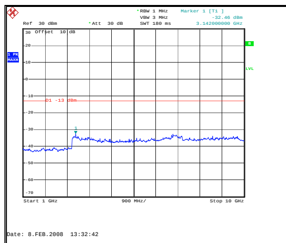
Figure 21: Spurious Emissions - Uplink CDMA Low Channel – Inter-modulation - 1 to 10 GHz
