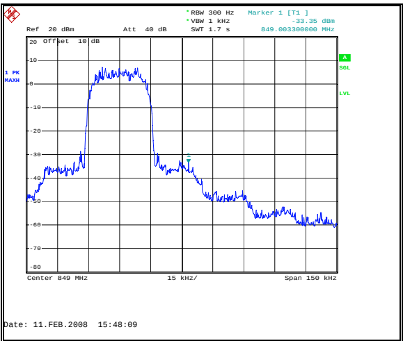
Figure 70: Band-Edge Uplink TDMA High Channel
