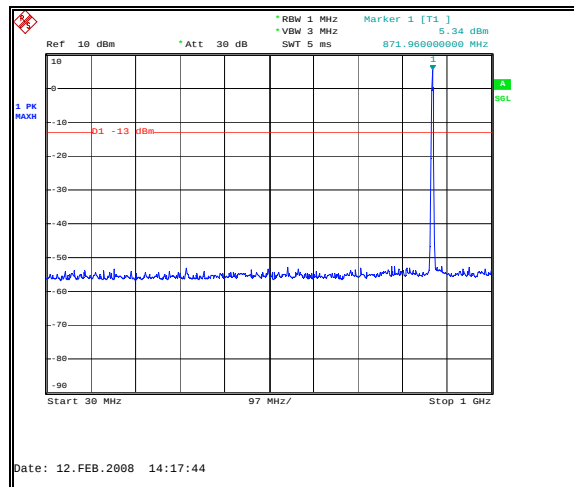
Figure 60: Spurious Emissions - Downlink GSM Low Channel – Inter-modulation - 30 MHz to 1 GHz
