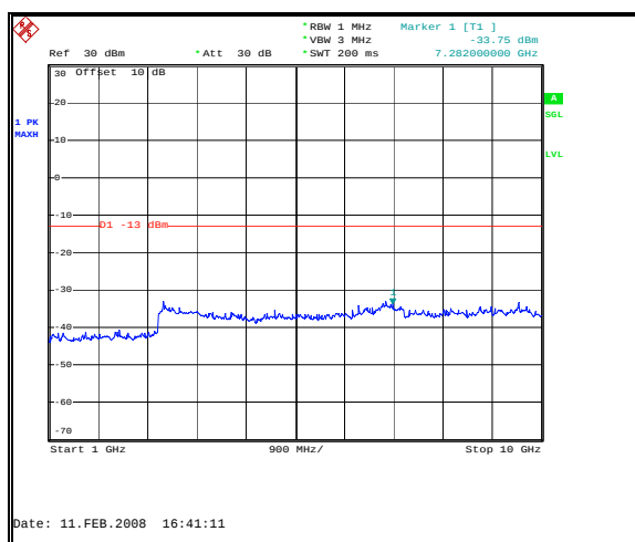
Figure 39: Spurious Emissions – Uplink GSM Mid Channel – 1 to 10 GHz
