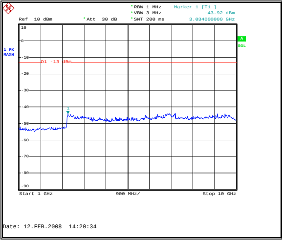
Figure 66: Spurious Emissions - Downlink GSM High Channel – Inter-modulation - 1 to 10 GHz
