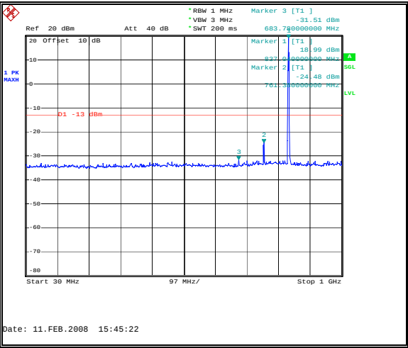
Figure 30: Spurious Emissions - Uplink TDMA Mid Channel – 30 MHz to 1 GHz
