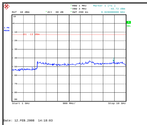
Figure 61: Spurious Emissions - Downlink GSM Low Channel – Inter-modulation - 1 to 10 GHz
