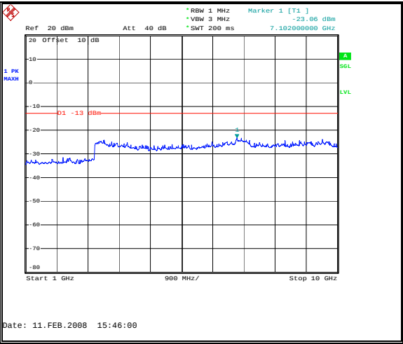
Figure 31: Spurious Emissions - Uplink TDMA Mid Channel – 1 to 10 GHz
