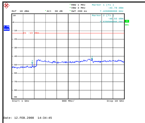
Figure 63: Spurious Emissions - Downlink GSM Mid Channel – 1 to 10 GHz
