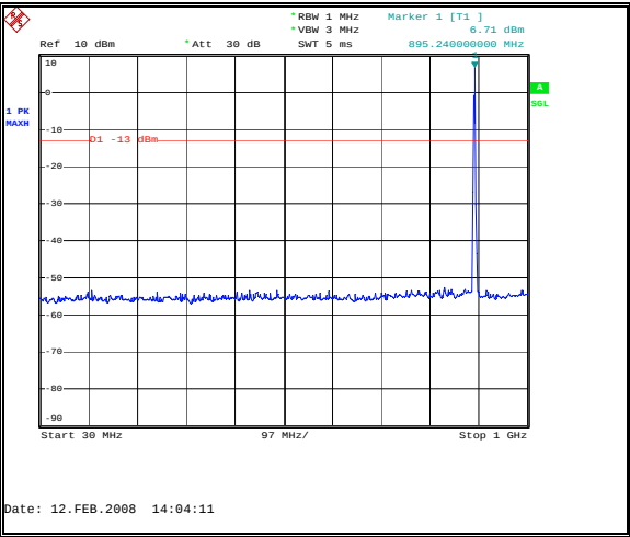
Figure 57: Spurious Emissions - Downlink TDMA High Channel –Inter-modulation-30MHz to 1GHz
