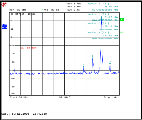
Figure 25: Spurious Emissions - Uplink CDMA High Channel – Inter-modulation - 30 MHz to 1 GHz
