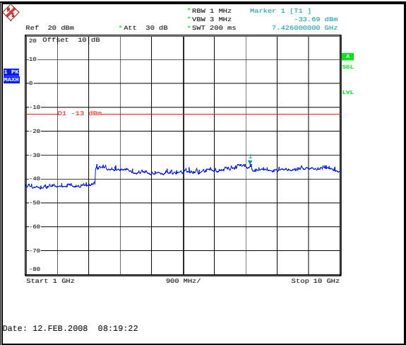
Figure 42: Spurious Emissions - Uplink GSM High Channel – Inter-modulation - 1 to 10 GHz
