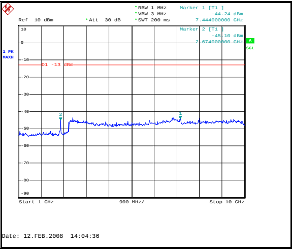
Figure 58: Spurious Emissions - Downlink TDMA High Channel – Inter-modulation - 1 to 10 GHz
