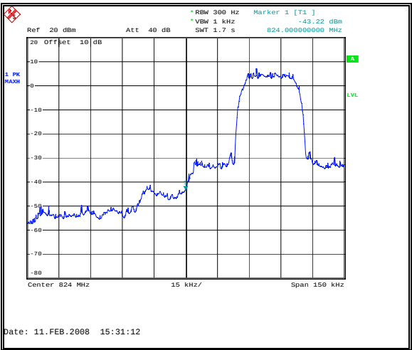
Figure 69: Band-Edge Uplink TDMA Low Channel
