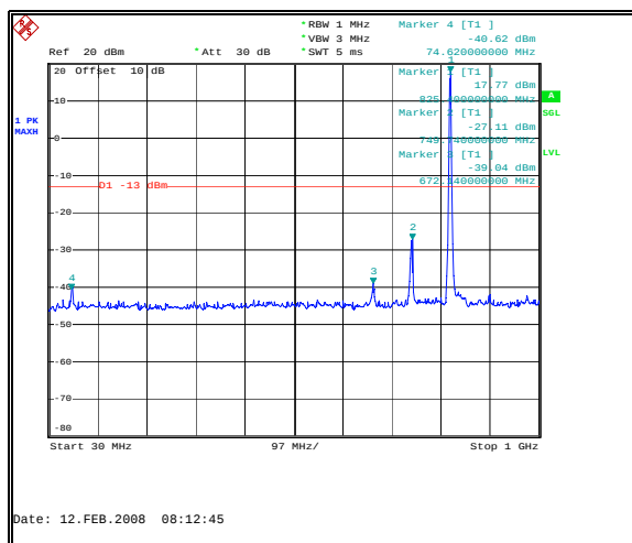
Figure 36: Spurious Emissions - Uplink GSM Low Channel – Inter-modulation - 30 MHz to 1 GHz
