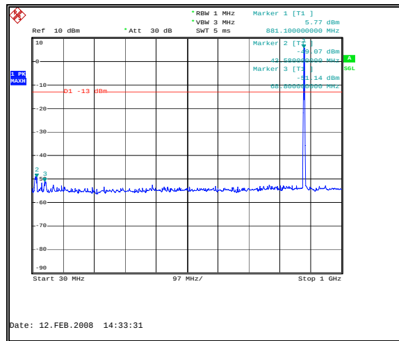
Figure 62: Spurious Emissions - Downlink GSM Mid Channel – 30 MHz to 1 GHz
