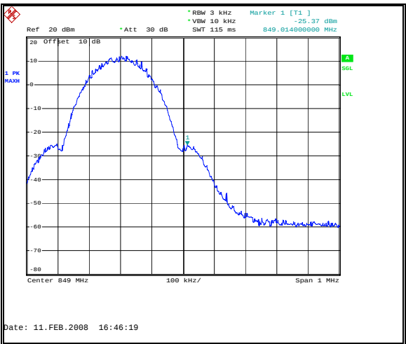
Figure 72: Band-Edge Uplink GSM High Channel
