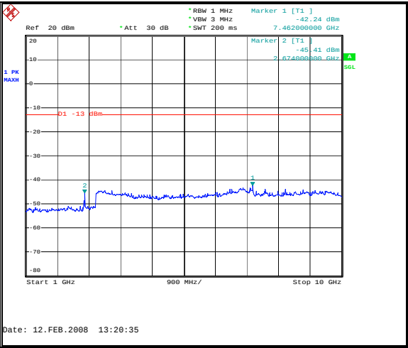
Figure 50: Spurious Emissions - Downlink CDMA High Channel – Inter-modulation - 1 to 10 GHz
