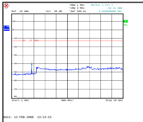
Figure 45: Spurious Emissions - Downlink CDMA Low Channel – Inter-modulation - 1 to 10 GHz
