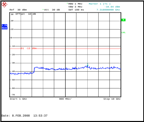
Figure 26: Spurious Emissions - Uplink CDMA High Channel – Inter-modulation - 1 to 10 GHz
