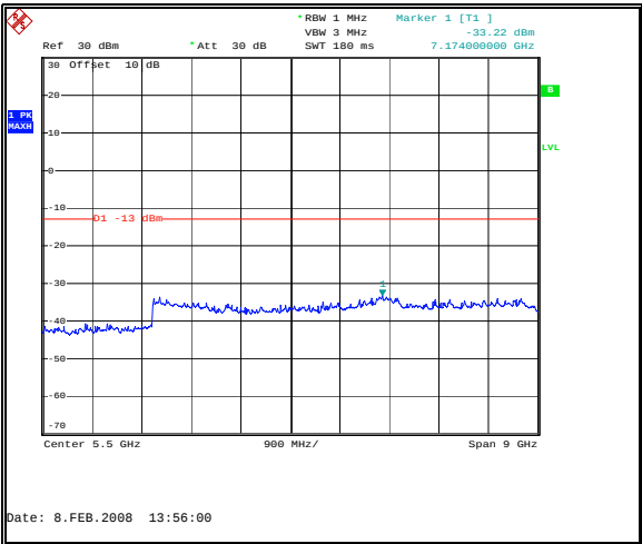
Figure 23: Spurious Emissions - Uplink CDMA Mid Channel – 1 to 10 GHz
