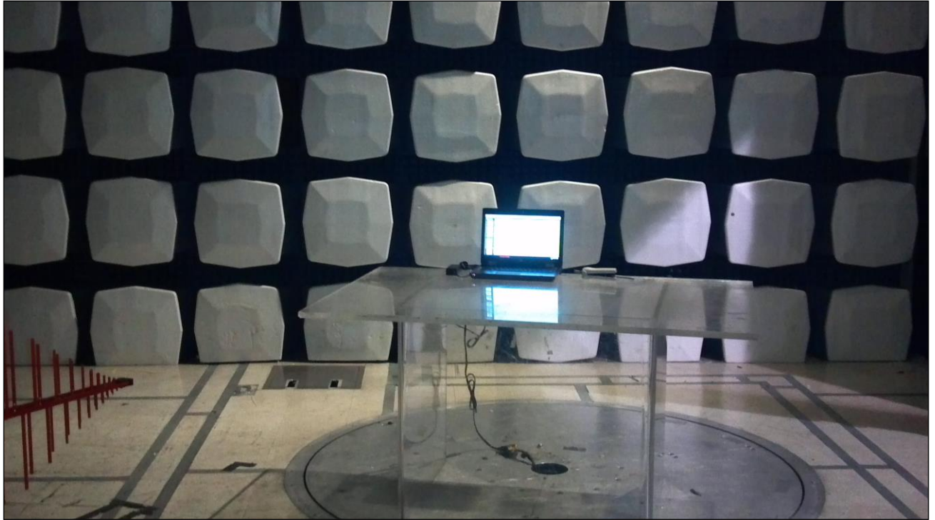
Photograph 4. Radiated Spurious Emissions, Test Setup, 30 MHz – 1 GHz
