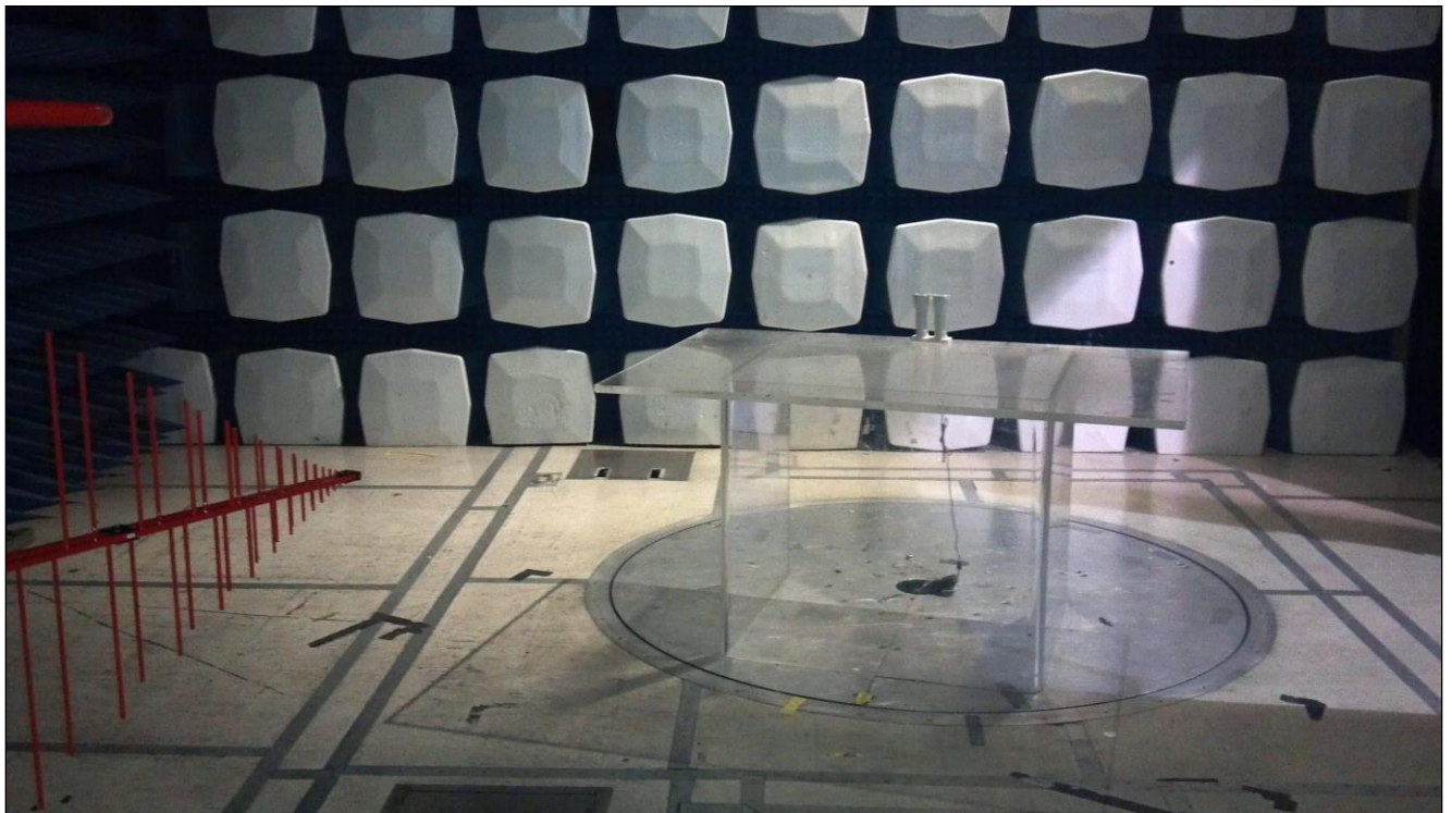
Photograph 3. Radiated Emissions, Test Setup
