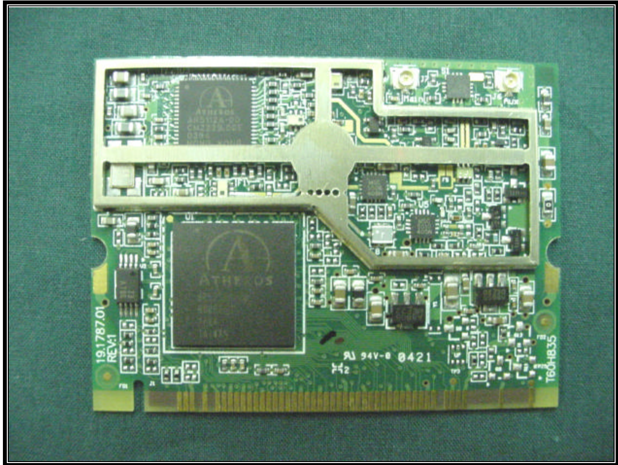
PHOTOGRAPH 16: WLAN TOP VIEW UNSHIELDED
