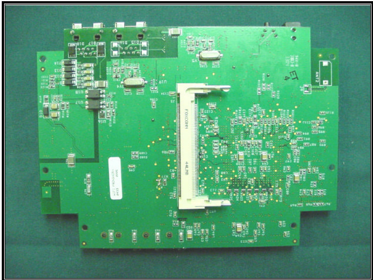
PHOTOGRAPH 13: INSIDE BOTTOM VIEW
