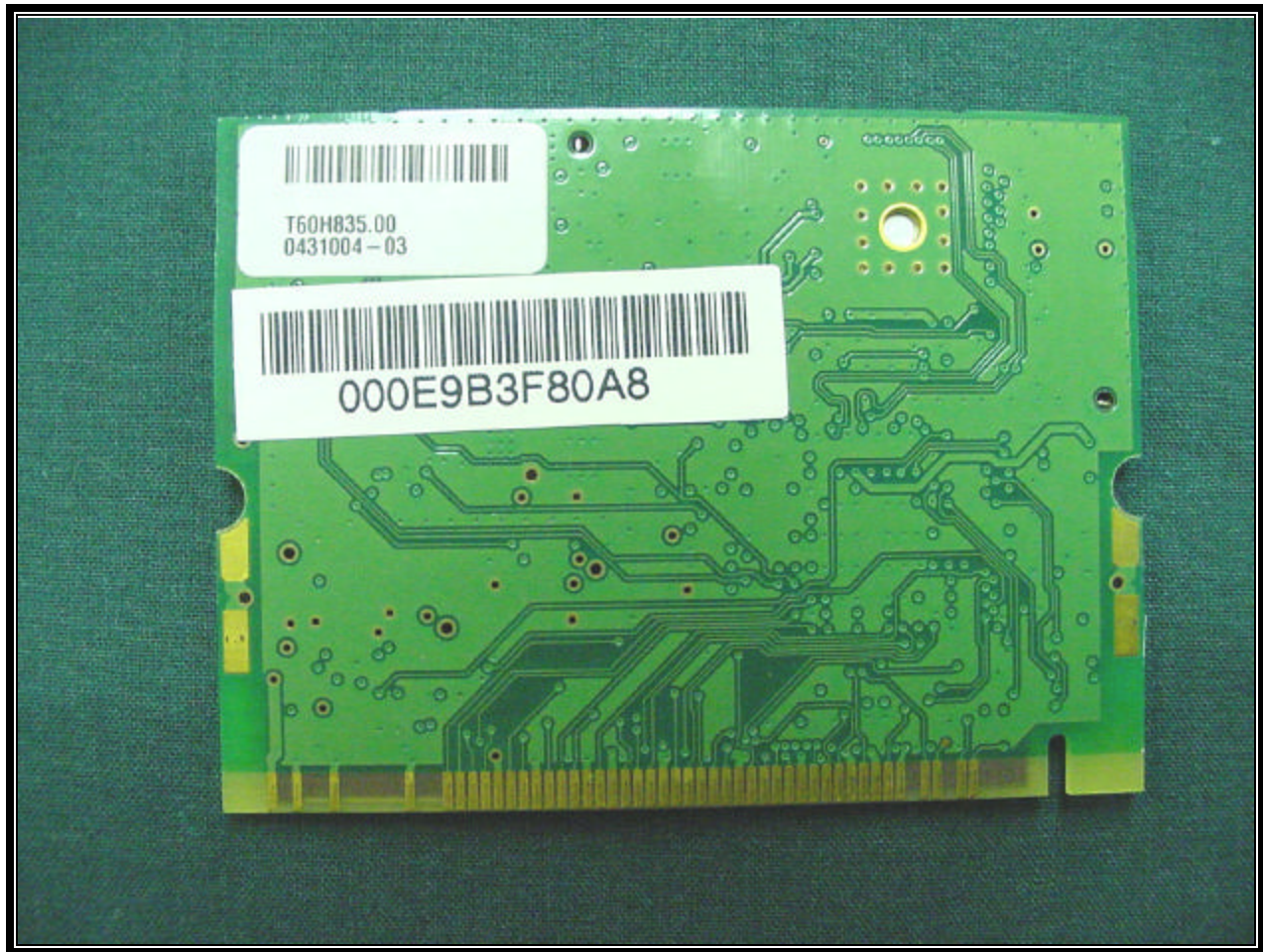
PHOTOGRAPH 15: WLAN BACK VIEW
