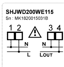
115V, connections
