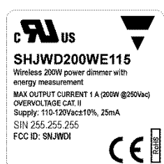
115V, product
