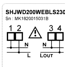
230V, black, light switch, connections
