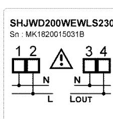
230V, white, light switch, connections
