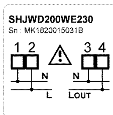
230V, connections
