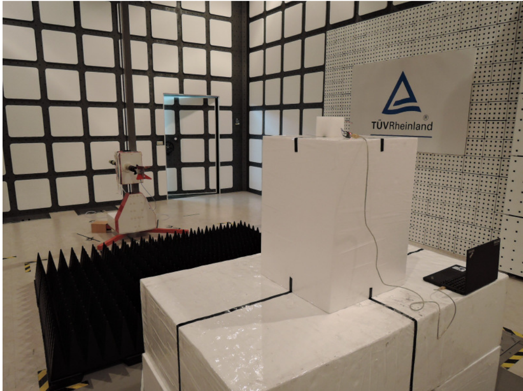
Photograph 2: Set-up for Fundamental and Spurious Emissions (Back View 1)
