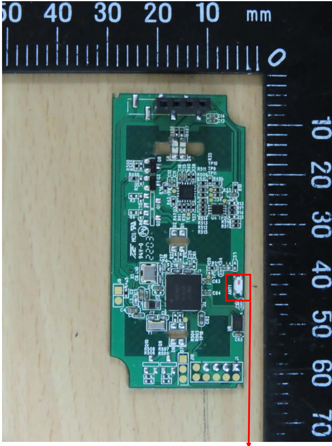
Multilayer Chip Antenna / Gain: 1.5 dBi
