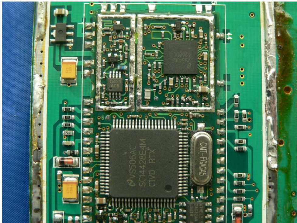
Base – RF shield off View 1
