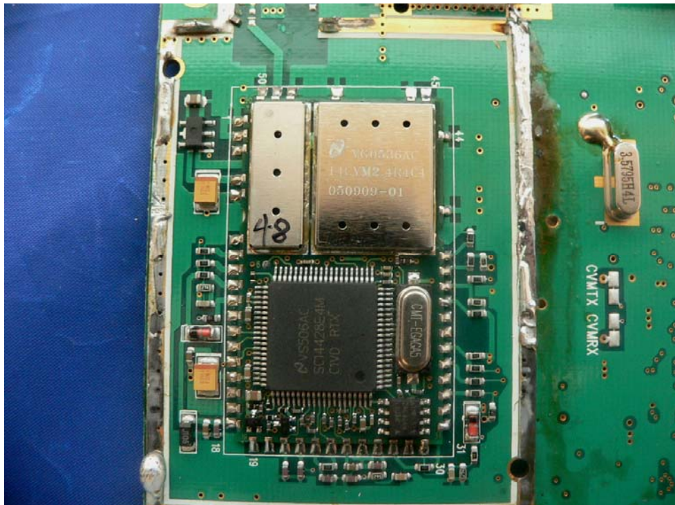
Base – 2.4GHz transceiver RF shield off View 1
