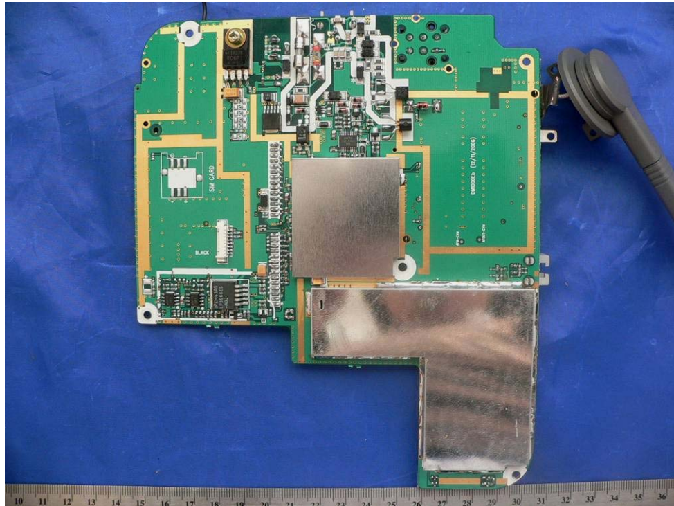
Base – Solder Side View
