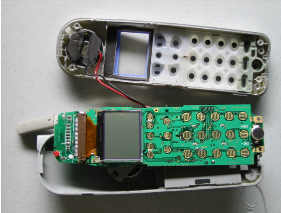
Handset – Dmode PCB Back View
