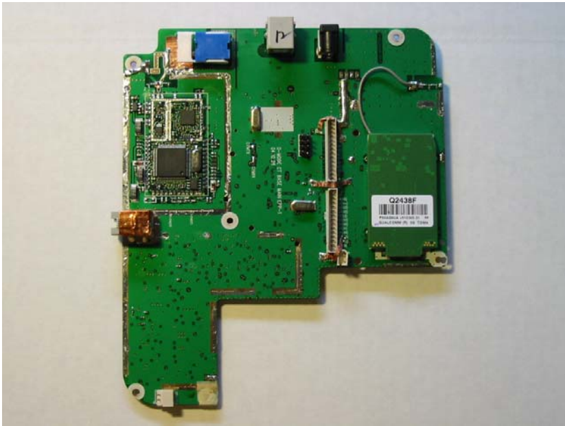
Base – Board Solder Shield Cover Removed View
