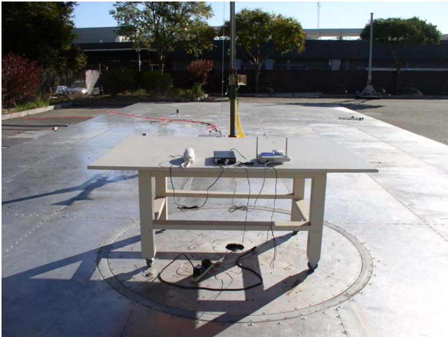
Base Radiated Emission – Rear View (2.4GHz FHSS)
