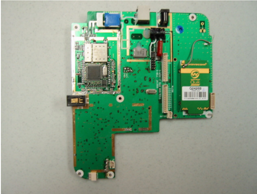
Base PCB Bottom View
