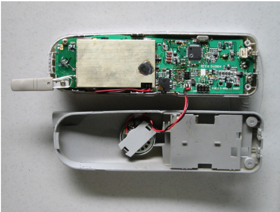
Dmode PCB HS Back
