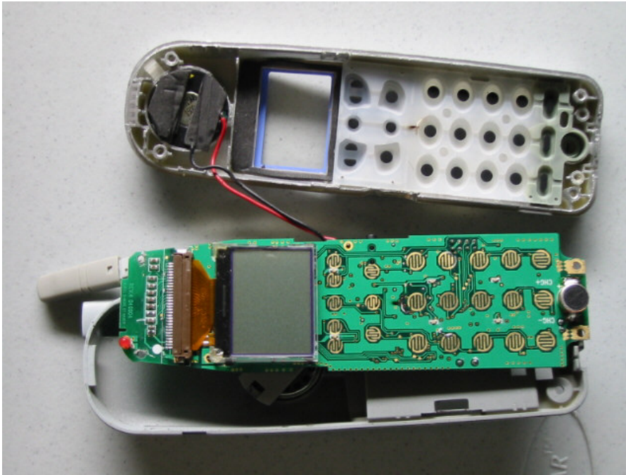
Dmode PCB HS front
