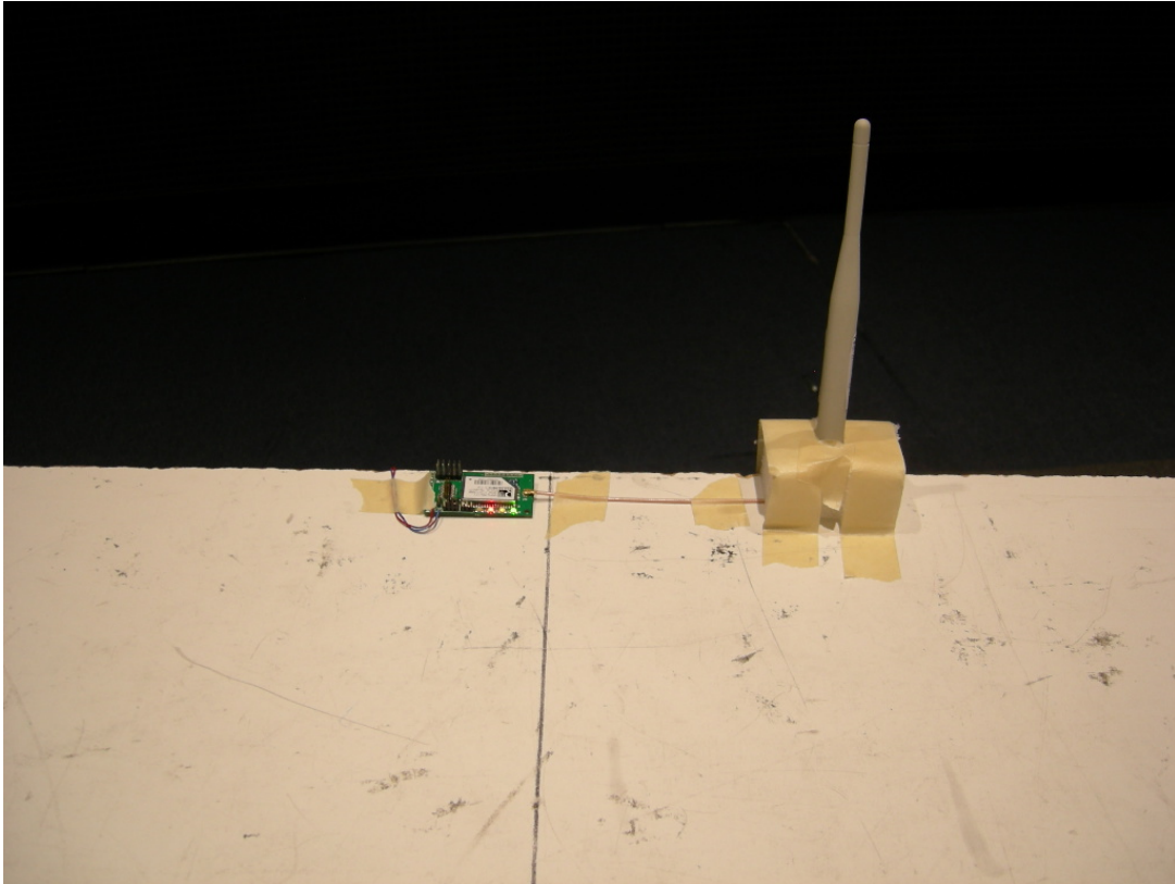
Figure 1: Radiated Emissions - XPOS
