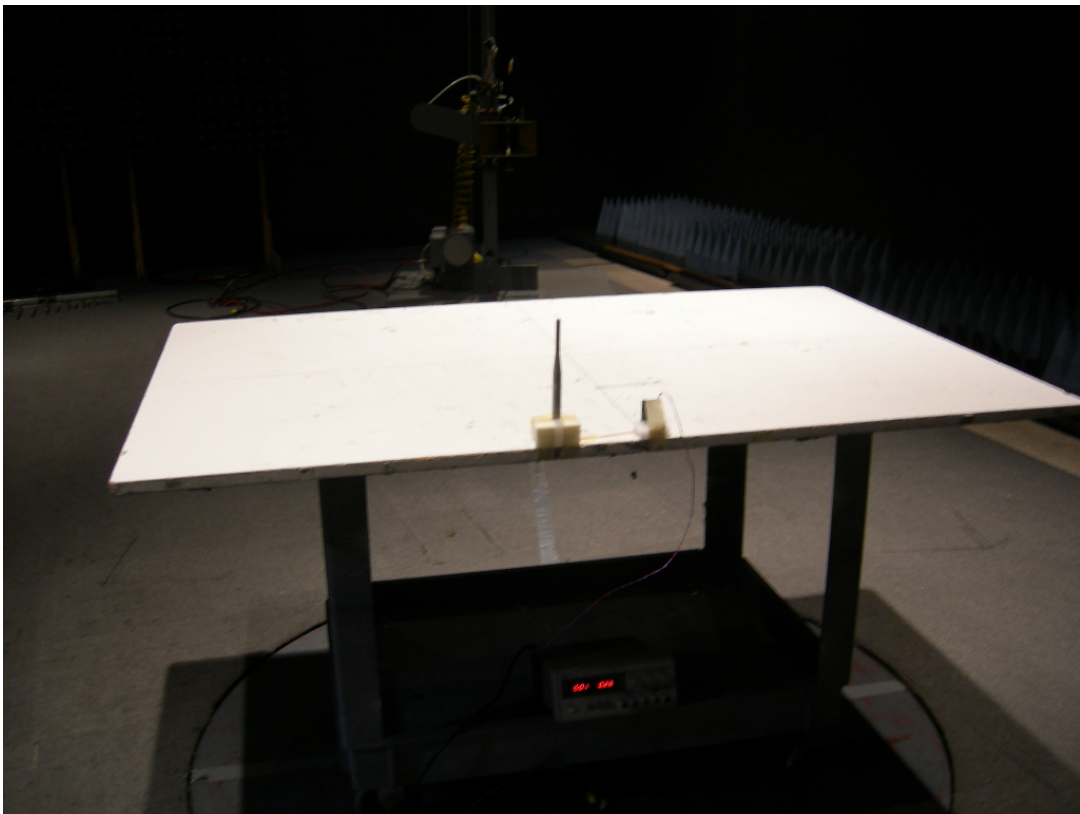
Figure 6: Radiated Emissions - ZPOS
