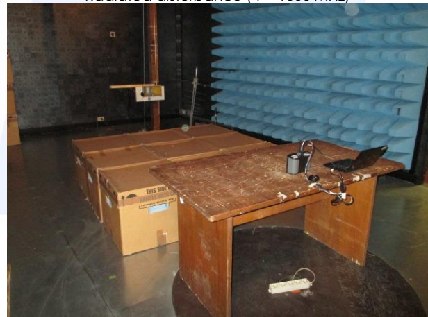
Radiated disturbance ( f > 1000 MHz)
