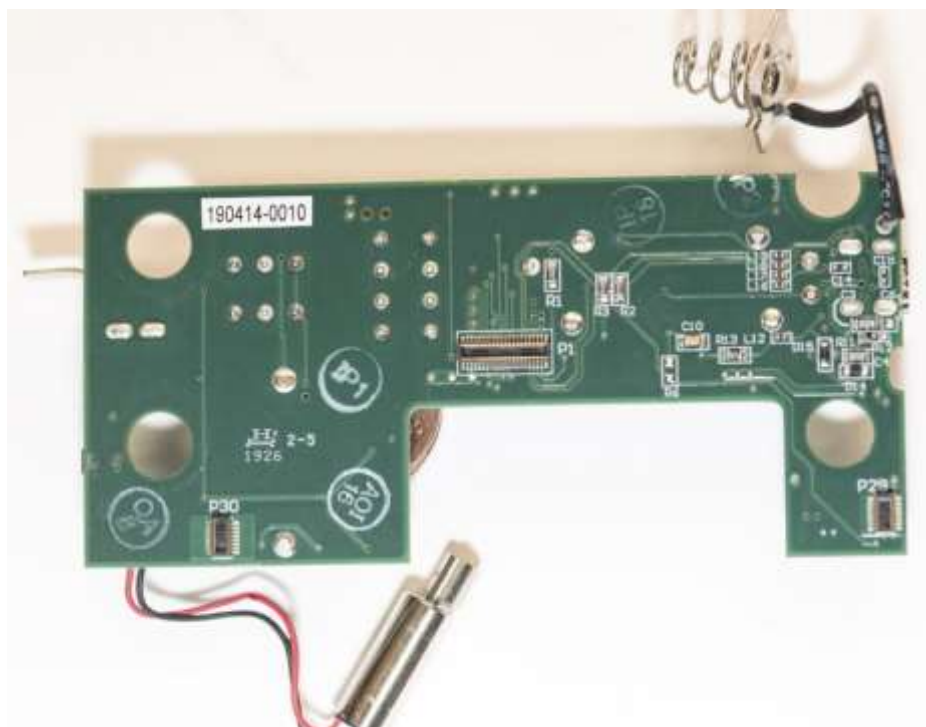
Fig 2.5. ENG 10001 204 Auxiliary Board, Bottom
