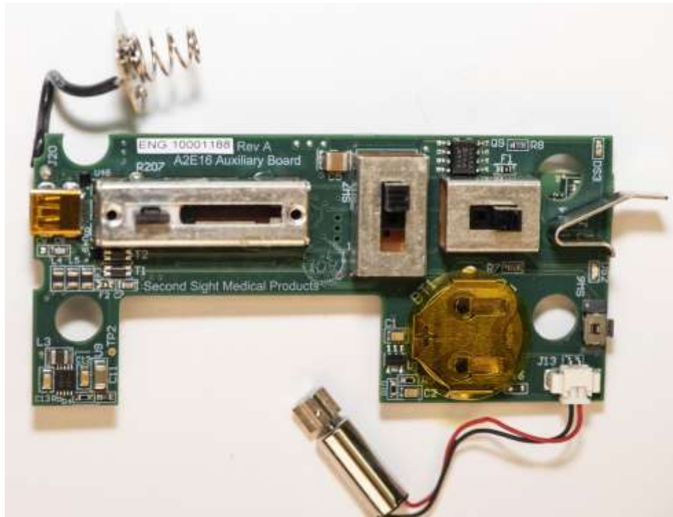
Fig 2.4. ENG 10001 204 Auxiliary Board, Top
