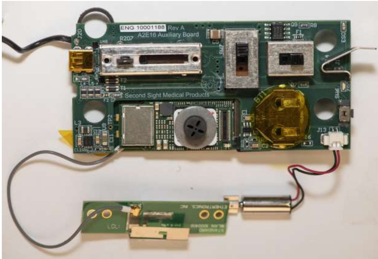
Fig 2.1. ENG 300300 663 VPU Main II Board Top with installed: ENG 10001 204 Auxiliary Board, and ENG 300300-608 SOM Board
