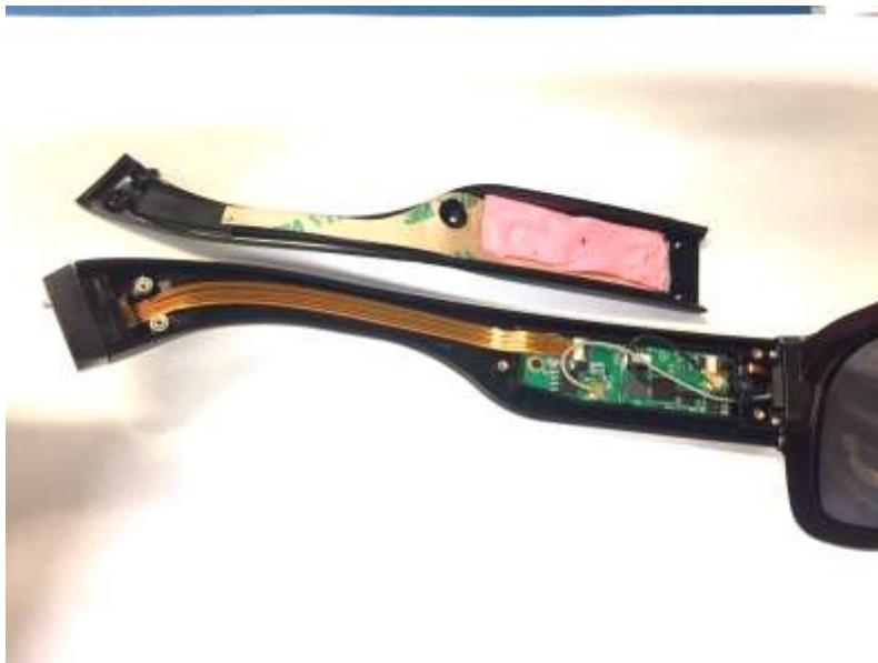
Fig 1.2. Interior view of Glasses RF electronics
