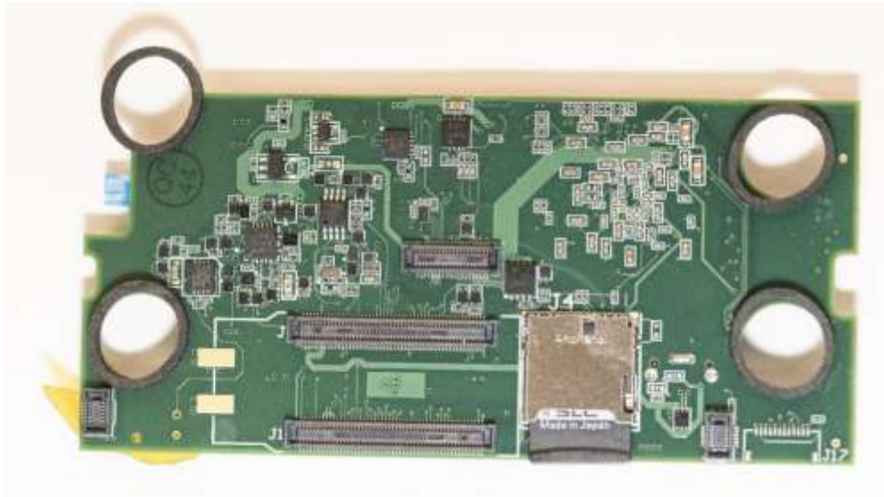
Fig 2.2. Part ENG 300300 663 VPU Main II Board Top (Auxiliary and SOM Boards Removed)
