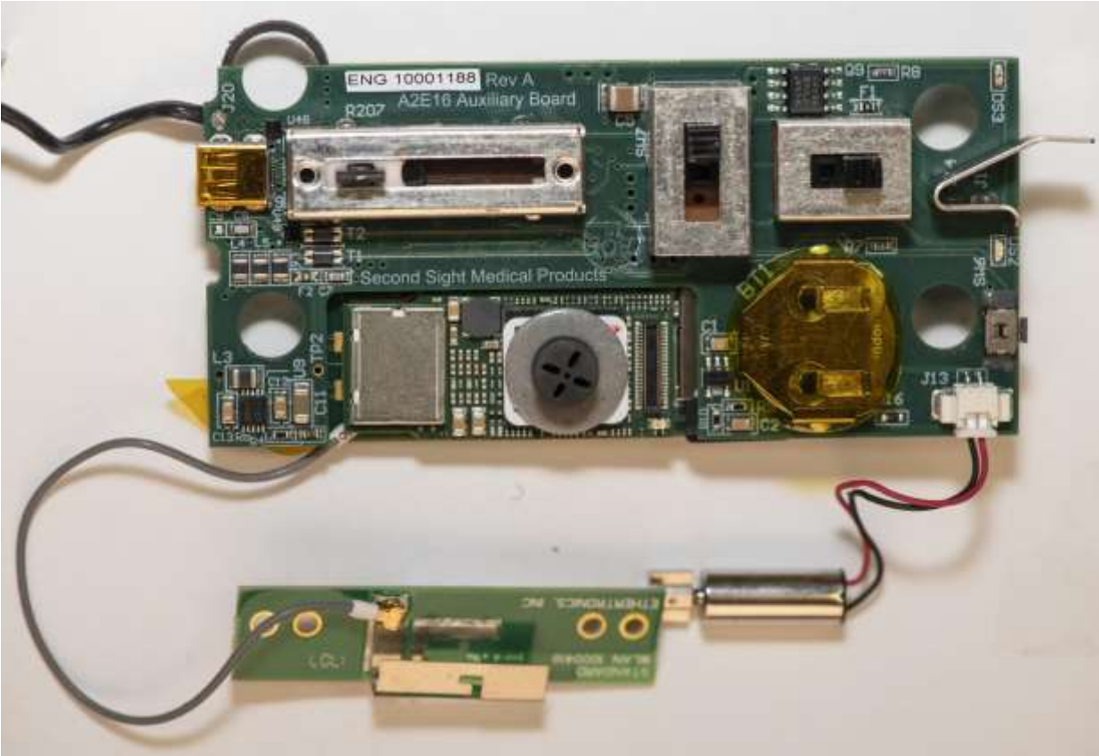
Fig 2.1. ENG 300300 663 VPU Main II Board Top with installed: ENG 10001 204 Auxiliary Board, and ENG 300300-608 SOM Board
