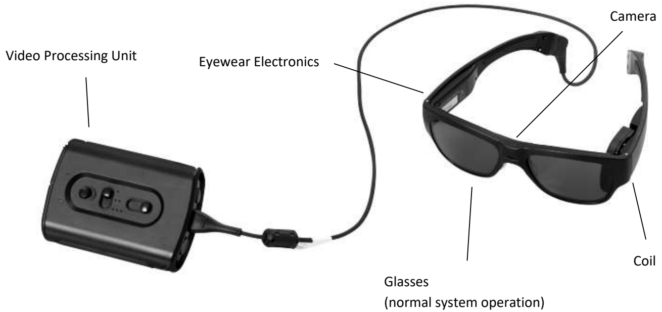
Figure 1. Argus 2s VPU (Video Processing Unit), Cable. and Glasses
