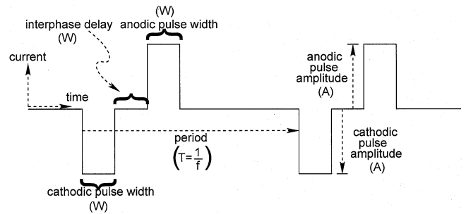
Fig. 5. Parameters of the biphasic current pulse used for retinal stimulation.
