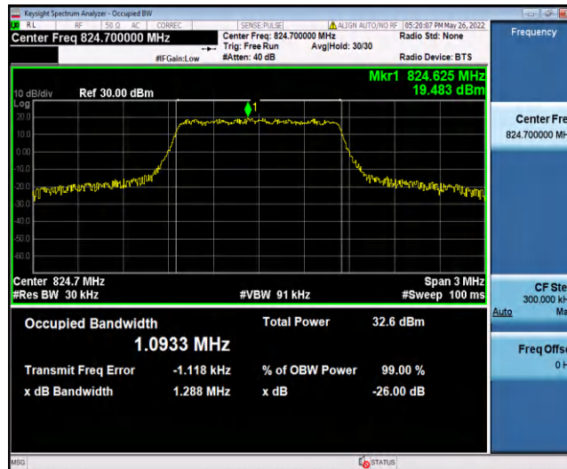
Band5-1.4MHz-QPSK-20407-6RB#0-1.0933
