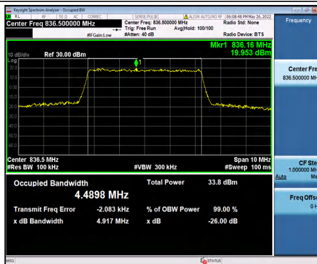
Band5-5MHz-QPSK-20525-25RB#0-4.4898
