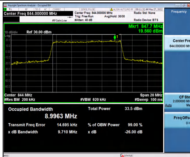
Band5-10MHz-16QAM-20600-50RB#0-8.9963
