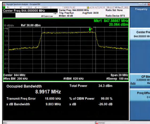
Band5-10MHz-QPSK-20600-50RB#0-8.9917
