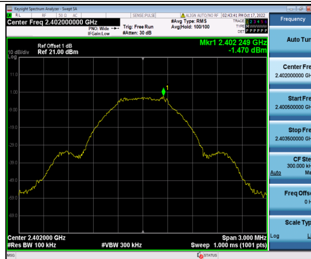
BLE_BT4.0_Ant1_2402_0~Reference
