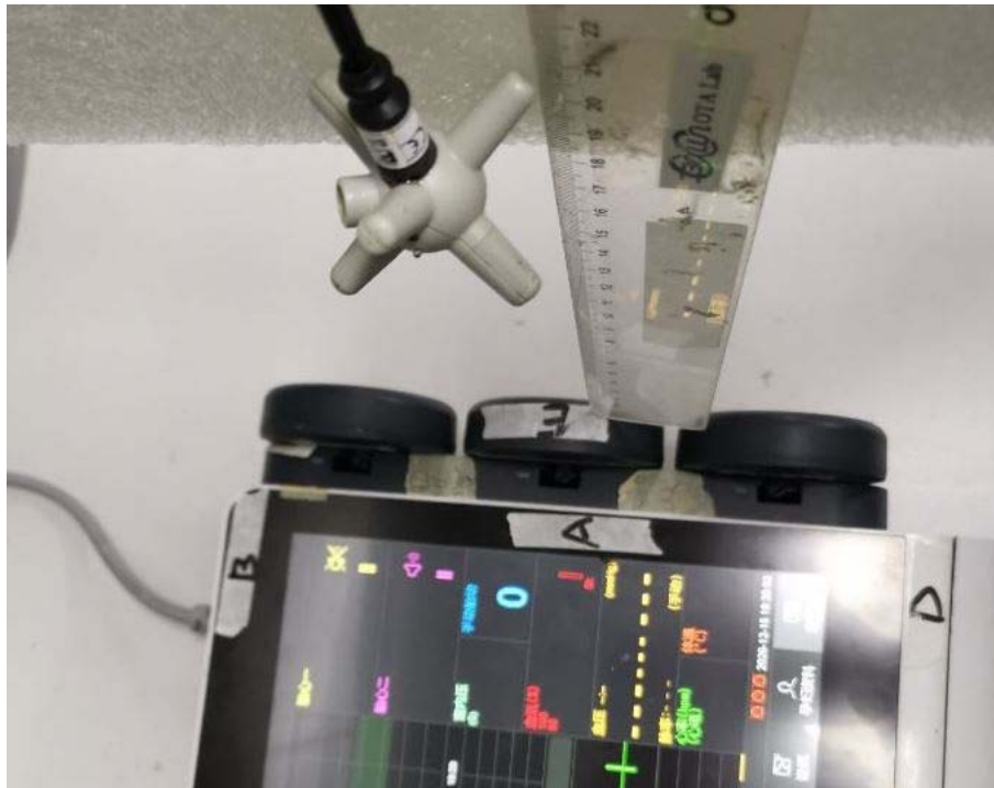
E-field Test Setup Photo of Position E(20cm)
